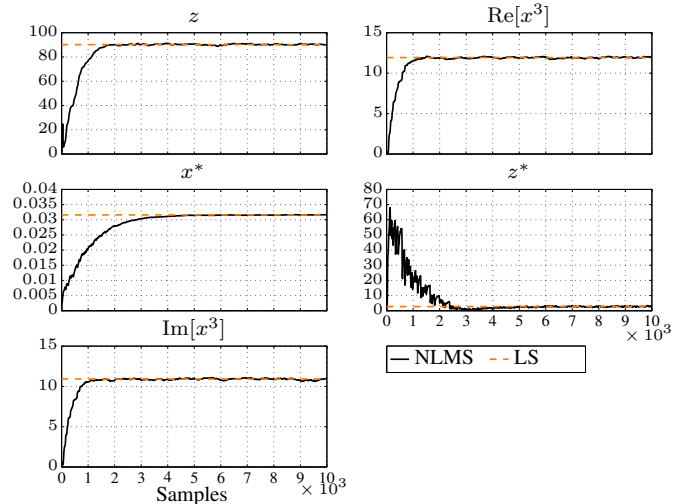
Fig. 11. Adaptation of the filter coefficients with BPSK input (magnitude of complex coefficients).
