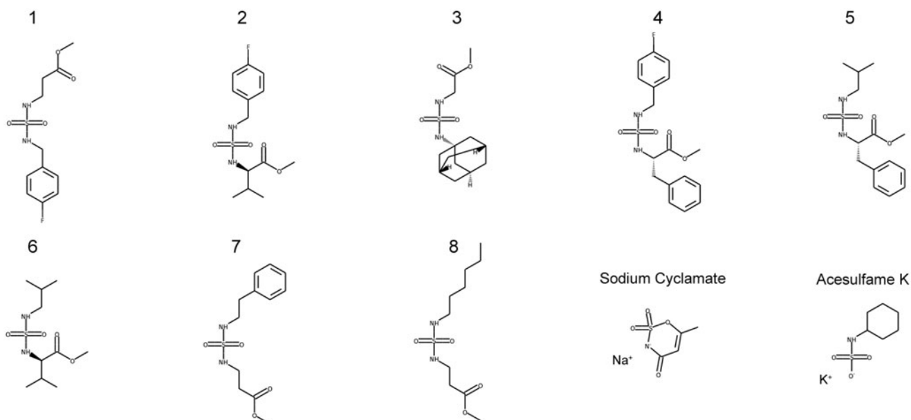
Figure 5. Candidates selected from the virtual screening.
