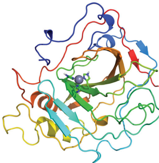
Figure 2. Final model of TcCA achieved from multi-template comparative modelling and subsequent iterative Rosetta-MD refinement. Histidine residues of the active site are highlighted in green for carbon atoms and in blue for nitrogen atoms. The zinc ion is represented as a non-bonded sphere in grey.
