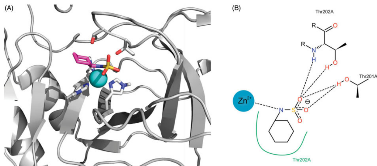
Figure 7. (A) Best docking solution for the interaction of cyclamate with the active site of TcCA . Histidine and important residues of the active site are highlighted in grey for carbon atoms, in red for oxygen atoms and in blue for nitrogen atoms. The zinc ion is represented as a non-bonded sphere in cyan. Colour code for cyclamate: Carbon atoms in violet, Nitrogen atoms in blue, sulphur atoms in yellow and oxygen atoms in red. (B) Schematic representation of the interactions between cyclamate and the active site of the TcCA model.
