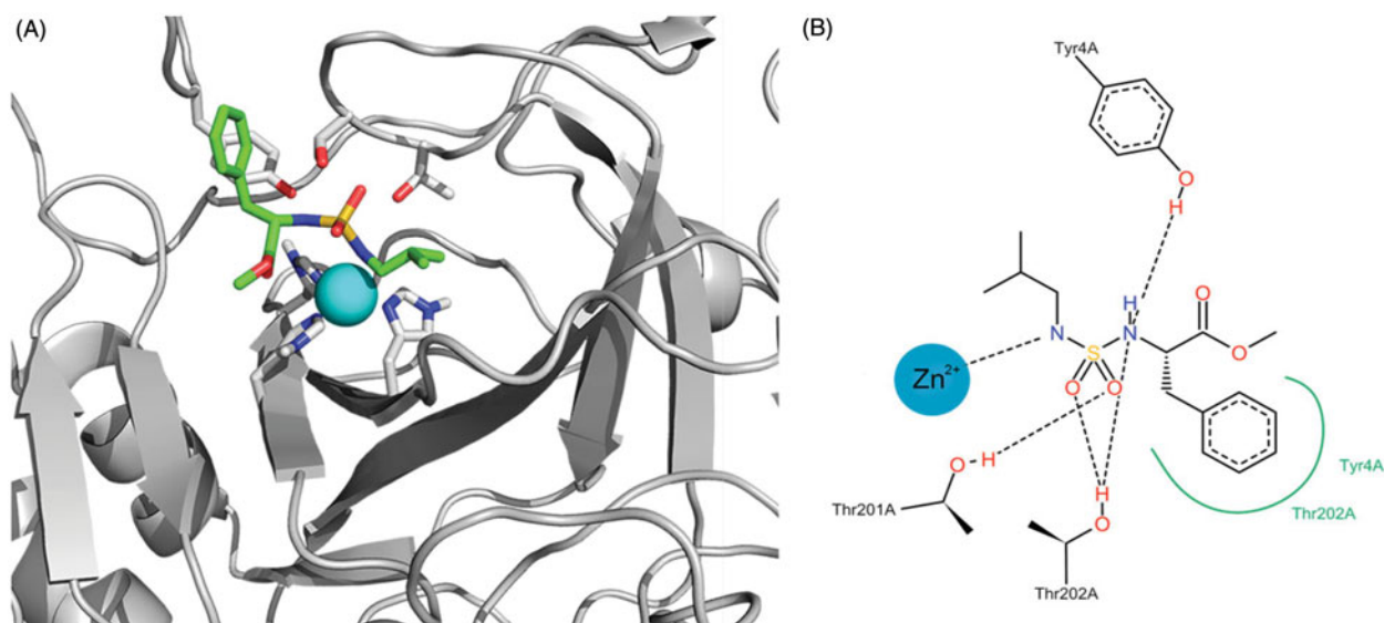
Figure 6. (A) Best docking solution for the interaction of compound 5 within the active site of TcCA. Histidine and important residues of the active site are highlighted in grey for carbon atoms, in red for oxygen atoms and in blue for nitrogen atoms. The zinc ion is represented as a non-bonded sphere in cyan. Colour code for compound 5 : Carbon atoms in green, Nitrogen atoms in blue, sulphur atoms in yellow and oxygen atoms in red. (B) Schematic representation of the interactions between compound 5 and the active site of the TcCA model.
