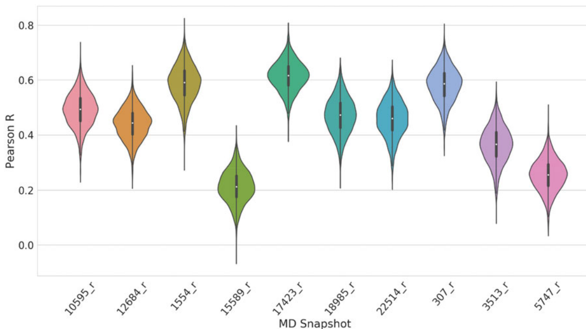
Figure 3. Pearson's R obtained from docking the validation set on every refined MD snapshot. The white dot represents the median value, and the black line height represents the distance between the lower quartile (Q1) to the upper quartile (Q3), which is called the interquartile range (IQR). Violin plots show the probability density of the data at different values as a kernel density estimation.
