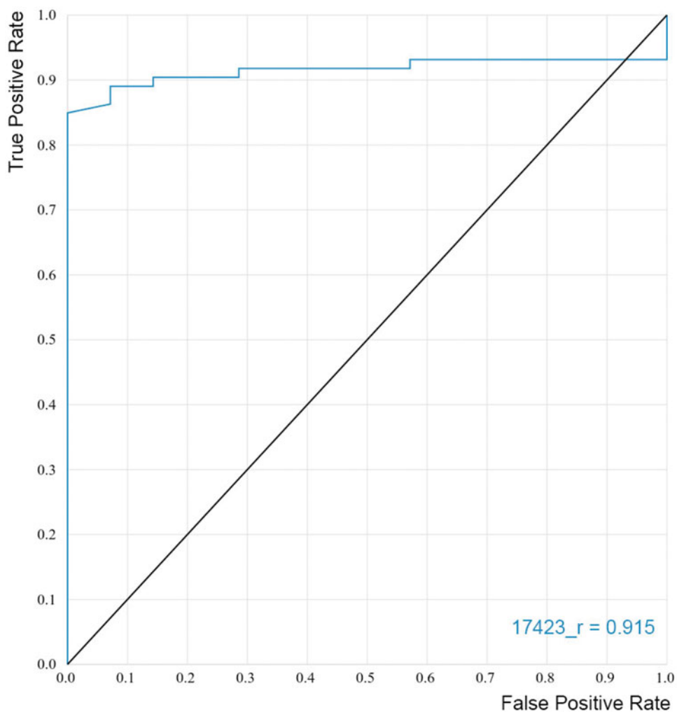
Figure 4. ROC curve obtained for the final model applied in the virtual screening.
