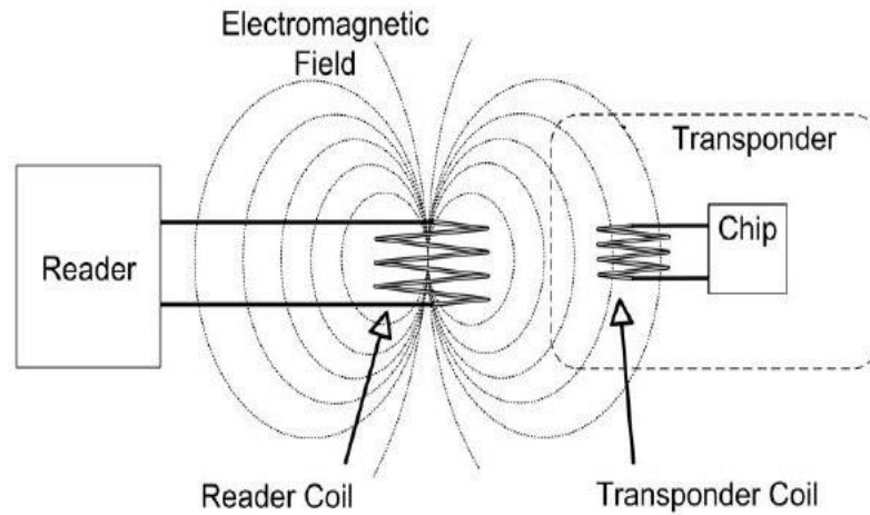
Figure 3 Induction between Tag and Reader in NFC /RFID
