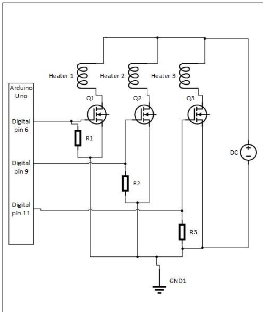
Figure 3. Schematic of the Arduino Proto Shield -circuit used to control the powers of the ceramic heating elements. The gate voltages of the MOSFETs (Q1, Q2, Q3) are controlled using analog voltage signals from three digital pins in Arduino Uno. According to the gate voltage, the heating power of the heaters change accordingly.
