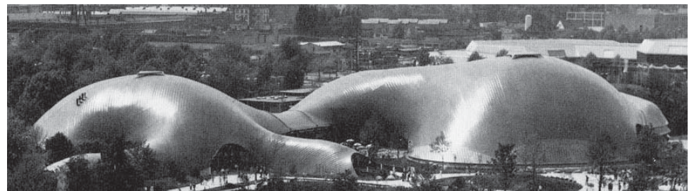
24 Mannheim Multihalle. A gridshell is a self-standing structure. The construction starts from a two-dimensional “grid mat”, which is deformed to an orthogonal grid three-dimensional grid. (Otto 1982, 49)
