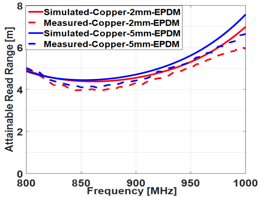
Figure 4.11. simulated and measured attainable read range of copper based RFID tag.
