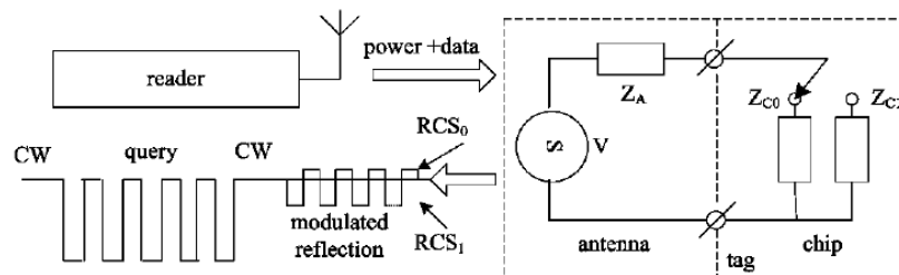
Figure 3.3 Passive backscatter RFID system [50].
