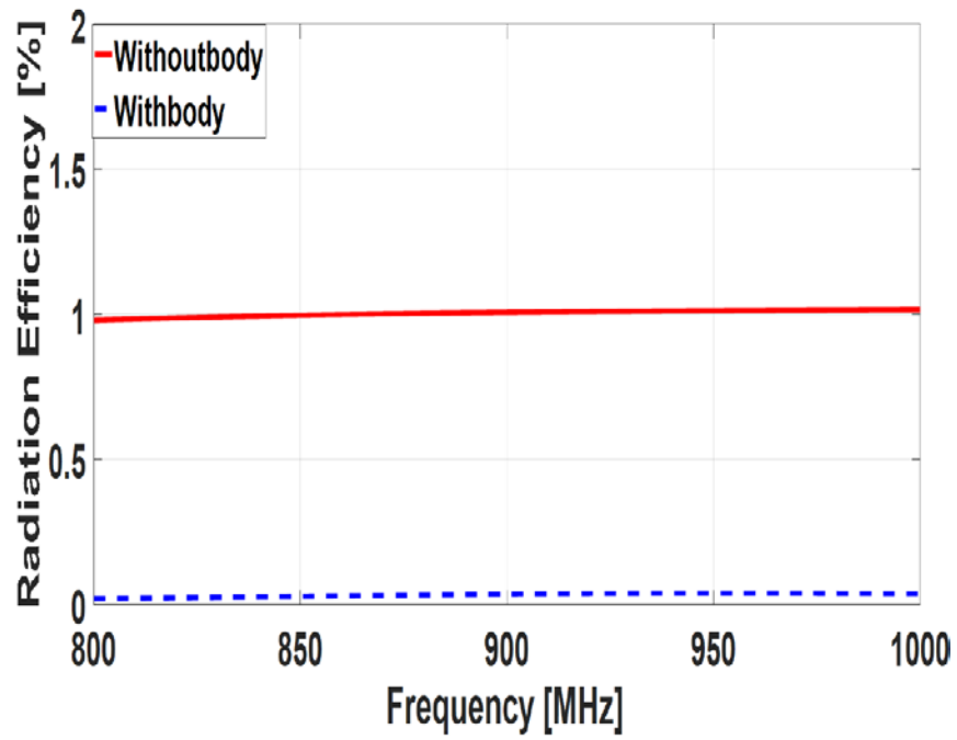
Figure 4.6 Radiation efficiency
