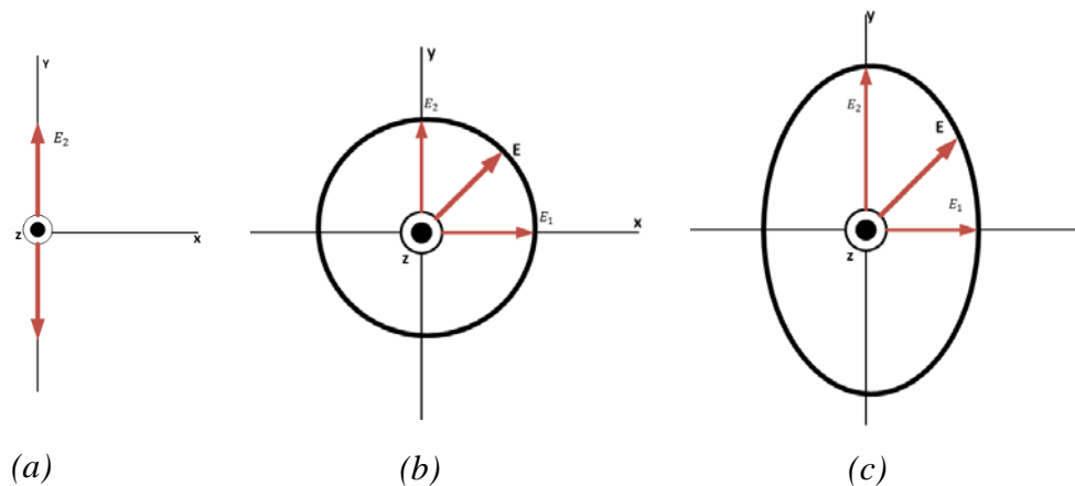
Figure 2.2 Polarization states
