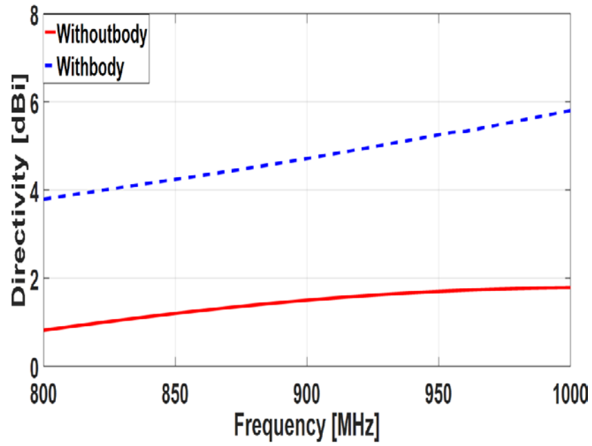
Figure 4.5 Directivity
