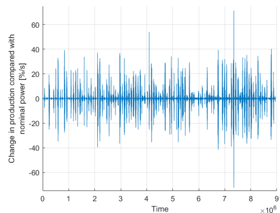
Figure 4 Changes in the PV production output power compared with nominal power of the solar PV system.
