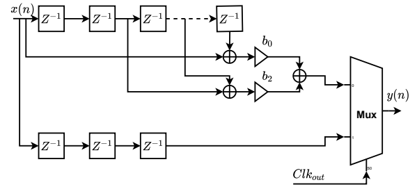
Fig. 6. Hardware Description of HBF
