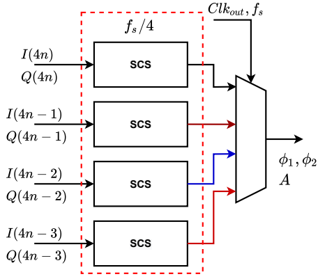
Fig. 8. Time Multiplexing of SCS
