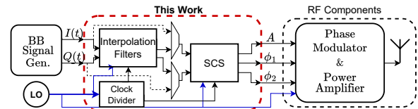
Fig. 1. Configurable DSP between Baseband (BB) Signal Generator and RF Components of a Transmitter.
