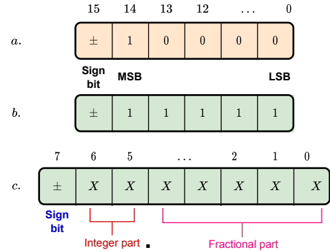
Fig. 10. Input data scaling a) Scaling used in this work, b) Full bit scaling, and c) Representation of fixed-point scaling with separate integer and fractional part of a given number.
