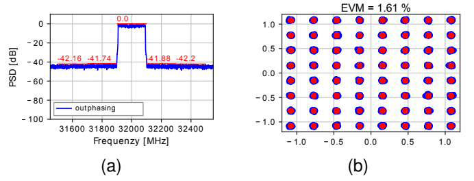
Fig. 9. a) ACLR & b) EVM performance of hardware DSP for an interpolation factor of 16
