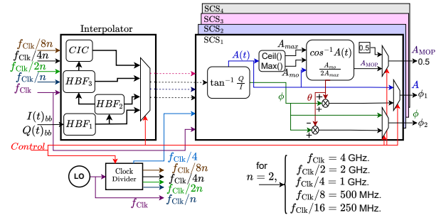
Fig. 3. High Level Functional block diagram of the proposed DSP
