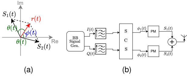
Fig. 2. Outphasing Modulation a) Outphasing vectors in complex plane, b) Generic block diagram of the outphasing transmitter
