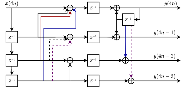
Fig. 7. Unrolling of Integrator by 4
