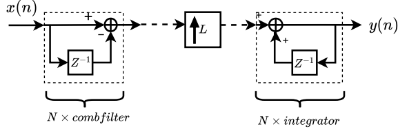
Fig. 4. Cascaded Comb-Integrator filter
