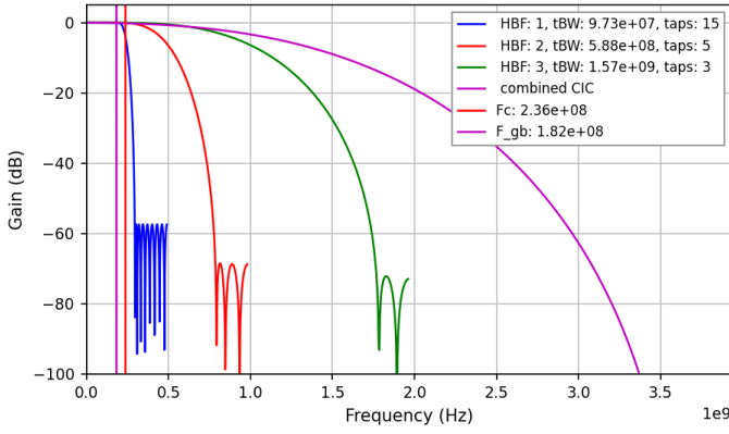
Fig. 5. Frequency Response of Filters
