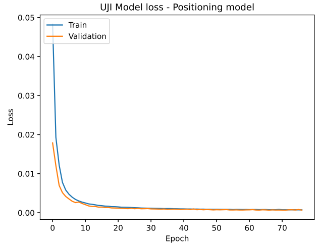
Fig. 4. CNN-LSTM model
