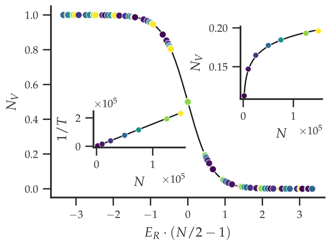
FIG. 2. Diagonal elements of the overlap matrix N_V , calculated numerically for system sizes ranging from N = 2006 (dark blue), through N = 20006, 25006, 50006, 75006, 100006 , and 125006 , to N = 150006 (yellow). To enable comparison between different system sizes, N_V is shown as a function of energy times the number of sites, E_R(N/2 - 1) such that it gives a constant temperature. The thermal Fermi-Dirac distribution of Eq. (5) (black line) can be clearly distinguished. The right inset shows the scaling of N_V with system size N for the first energy level above zero. The black line is the best fit N_V = 0.019 \log(N) - 0.032 . While the left inset indicates the linear scaling of \beta = 1/T with system size N , the black line is the continuous expectation 1/T = \frac{\lambda(N/2-1)}{\pi} .
