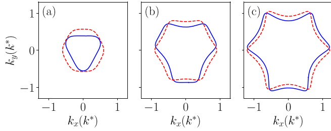
FIG. 2. (a)–(c) Fermi contour for Fermi energies E_F/E^* = 0.6, 0.9, and 1.2 . Dashed red and solid blue curves correspond to \Theta -symmetric ( \Delta/E^* = 0 ) and \Theta -broken ( \Delta/E^* = 0.4 ) cases, respectively.
