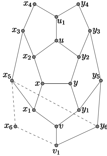
FIGURE 7. The graph for case 2 b) with iii), vi) and vertices v_1 and y_6 have two possible ways to continue
