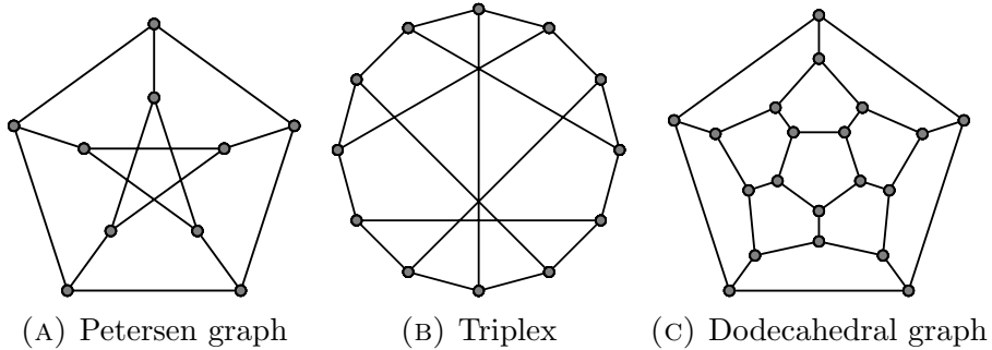
FIGURE 1. The three Ricci-flat cubic graphs with girth 5
