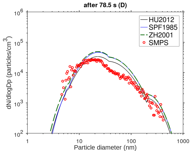
Figure E2. Modelled particle number size distribution with MAFOR using different dry deposition parameterizations at point D (after 78.5 s of plume transport time). HU2012 is the reference dry deposition configuration used in MAFOR, SPF1985 is the dry deposition scheme in AEROFOR, and ZH2001 is the dry deposition scheme in SALSA. Measured size distributions from SMPS are shown as red circles.
