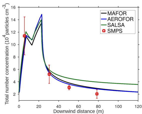
Figure 10. Comparison of total particle number concentrations as a function of downwind distance in the Urban Case scenario. Model results from the aerosol dynamics models MAFOR, AEROFOR, and SALSA. Measurement data from SMPS at points A, B, C, and D (error bars indicate 1\sigma standard deviation).
