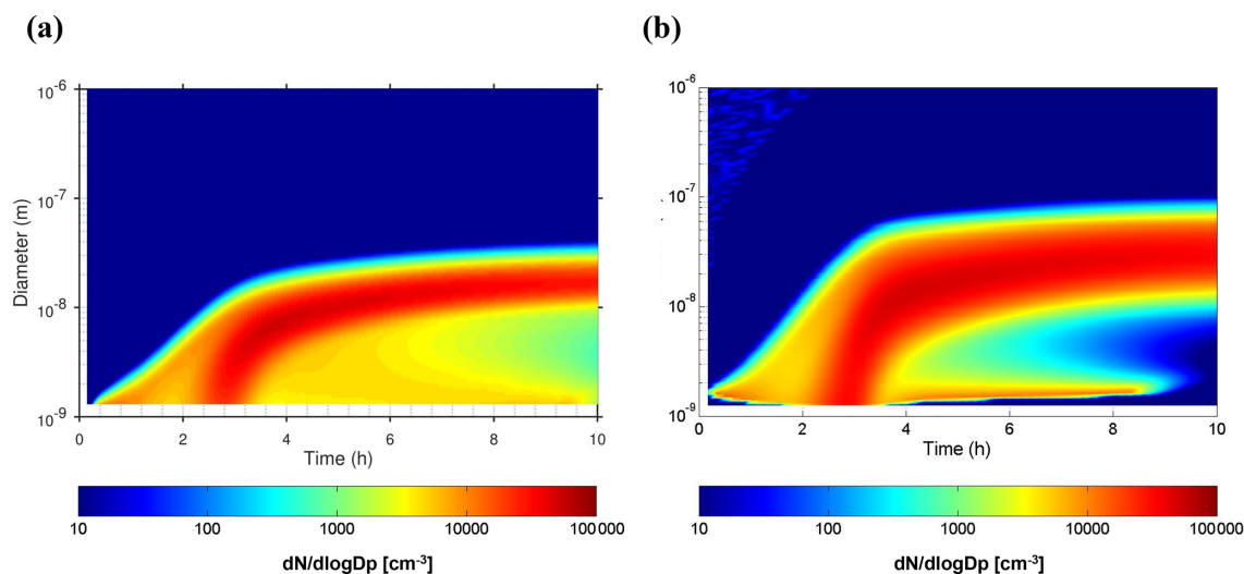
Figure 15. Evolution of the modelled particle number size distribution in a 10 h simulation to compare the performance of the nucleation code M2018 in (a) MAFOR v2.0 to that in (b) AEROFOR. New particles were inserted at 1.0 and 1.5 nm diameter in MAFOR and AEROFOR, respectively. The first particle formation after 15 min is due to ion-induced nucleation, and the main particle burst after 2 h is due to neutral nucleation. Final mean D_p was 18 and 22 nm, respectively, in MAFOR and AEROFOR simulations. Details on the configuration of the numerical experiment are given in Appendix H.
