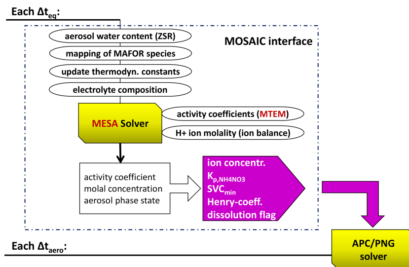
Figure 6. Workflow of the dynamic partitioning of semi-volatile inorganic gases. The MOSAIC interface is called every \Delta t_{\text{eq}} = 120 s, while the PNG solver is called every time step of the aerosol dynamic solver ( \Delta t_{\text{aero}} ). The MOSAIC interface outputs the gas–solid equilibrium coefficient for ammonium nitrate, the minimum saturation vapour concentration ( \text{SVC}_{\text{min}} ), the effective Henry’s law coefficient, the ion concentrations, and a dissolution flag (indicating if a solid is present in a size bin or not) for each size bin of the particle population.
