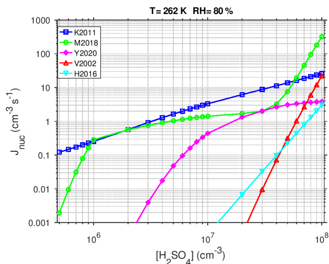
Figure 2. Predicted nucleation rate J_{\text{nuc}} ( \text{cm}^{-3} \text{ s}^{-1} ) as a function of the concentration of \text{H}_2\text{SO}_4 (at T = 262 \text{ K} and \text{RH} = 80 \% ) calculated with different parameterizations for particle formation through sulfuric acid: combined activation and IMN (K2011), neutral and ion-induced BHN (M2018), TIMN at [\text{NH}_3] = 1 \times 10^5 \text{ cm}^{-3} (Y2020), THN at [\text{NH}_3] = 2 \times 10^6 \text{ cm}^{-3} (H2016), and classical BHN (V2002).
