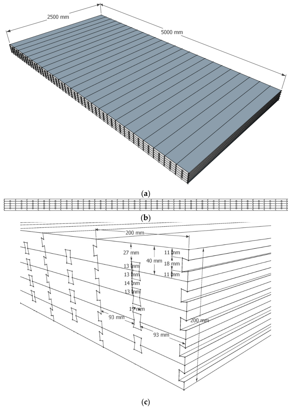
Figure 5. Dovetail wood board elements as floor slab alternative 2 (key-type): (a) isometric view, (b) side view, (c) with representative dimensions.
