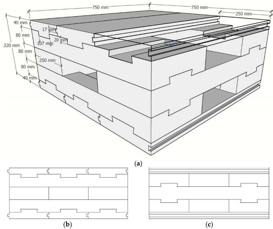
Figure 7. Dovetail wood board elements as floor slab alternative 4 (hollow-type-2): (a) isometric view with dimensions, (b) front view, (c) side view.
