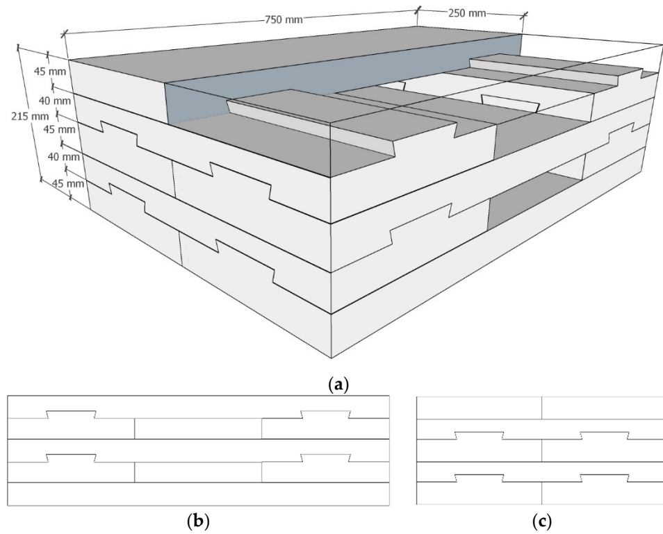
Figure 6. Dovetail wood board elements as floor slab alternative 3 (hollow-type-1): (a) isometric view with dimensions, (b) front view, (c) side view.
