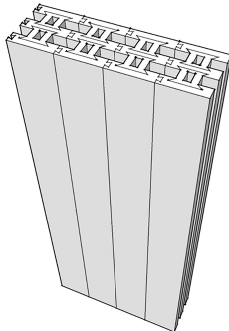
Figure 9. Dovetail wood board elements as shear wall alternative 2 (hollow-type 2).
