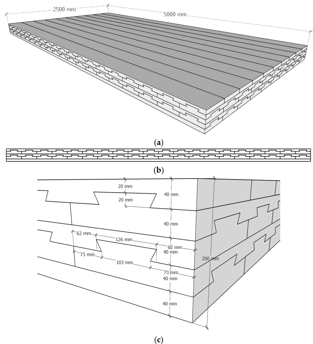
Figure 4. Dovetail wood board elements as floor slab alternative 1 (solid/massive-type): (a) isometric view, (b) side view, (c) with representative dimensions.
