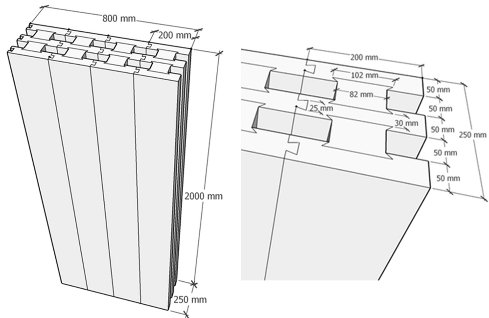
Figure 8. Dovetail wood board elements as shear wall alternative 1 (hollow-type 1) (isometric views with dimensions).
