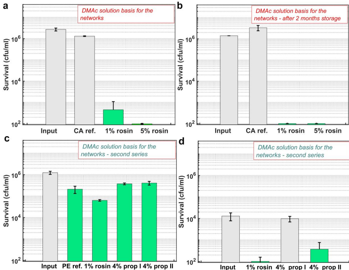
Fig. 7. Antibacterial activity of electrospun fiber networks against S. aureus : a) DMAC solvent systems; b) DMAC solvent systems after two months; c) second series DMAC solvent systems; d) second series DMAC solvent systems for a lower input of bacteria. The analysis was carried out for approximately 1 cm by 1 cm samples (approximately 1.3 to 2.5 mg) in liquid (Ringer's medium, 1/4 strength) and after 24 h of mixing at room temperature. The analysis resolution is 100 cfu per mL. Pure CA and polyethylene (PE) fibers were used as the reference.
