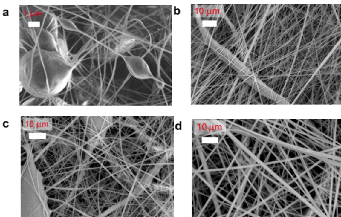
Fig. 2. Electrospun CA fiber networks with various rosin or propolis concentrations: a) CA (10%) rosin 5% in DMAc basis; b) CA (10%) propolis II 5% in DMAc basis; c) CA (10%) rosin 1% in DMAc basis; d) CA (10%) rosin 5% in DMAc basis
