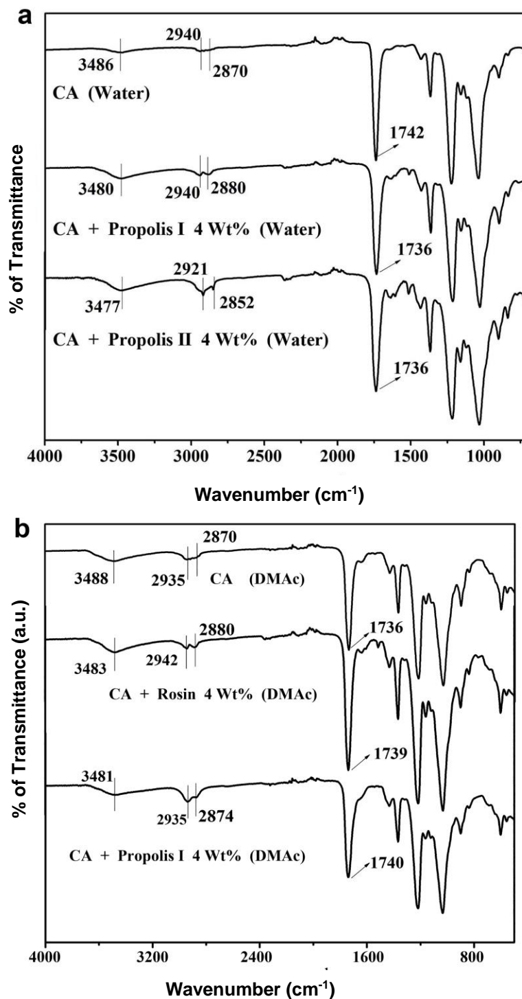
Fig. 5. FTIR spectra of electrospun CA fibers with rosin and propolis contents: a) propolis containing fiber networks (H 2 O basis); b) propolis and rosin containing fiber networks (DMAc basis)
