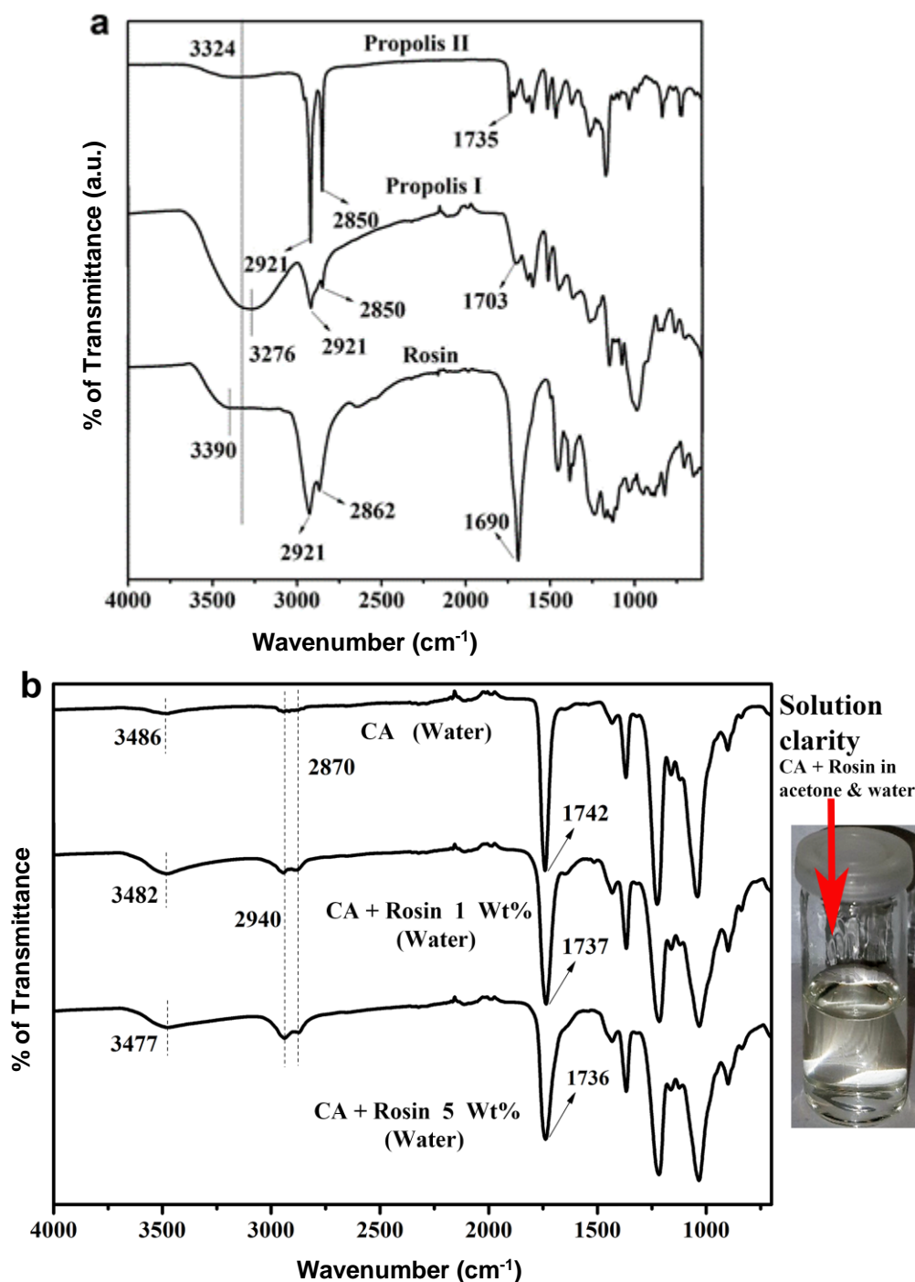
Fig. 4. FTIR spectra of the raw materials used and electrospun CA fibers: a) raw materials; b) electrospun CA fibers with rosin ( \text{H}_2\text{O} basis)
