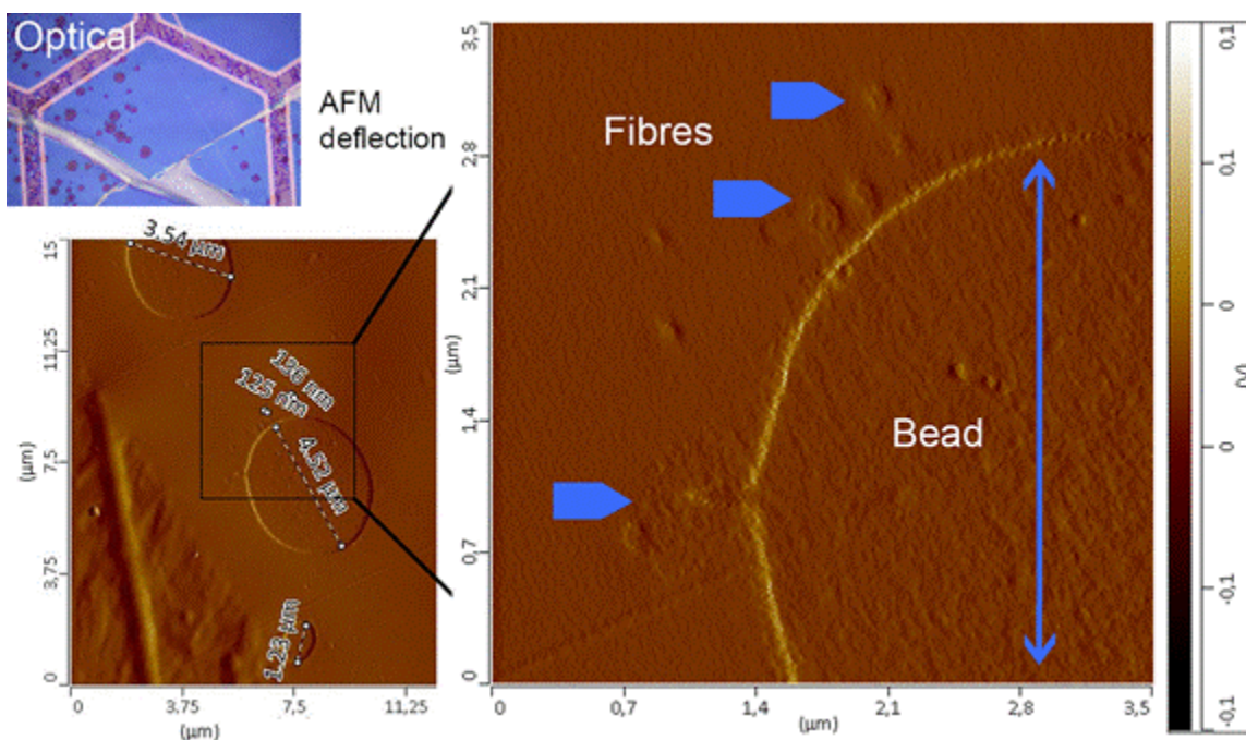
Fig. 3. AFM analysis of the CA-rosin electrospun network and the fiber and beaded cross sections. The measurements were done in contact mode using an Au coated silicon probe. The ultra-microtomed slices including the electrospun network sample were laid on TEM grids with a carbon film.
