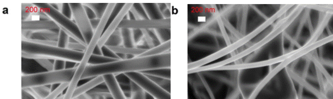
Fig. 1. Electrospun pure CA fiber networks based on either DMAc or H 2 O solution: a) CA (10%) in H 2 O basis; b) CA (5%) in DMAc basis
