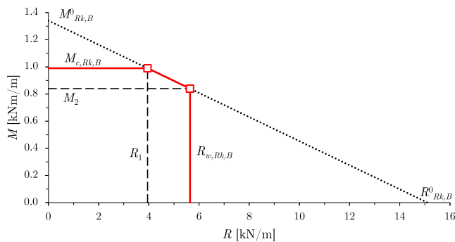
Fig. 18. M/R -interaction: Sin-46/150, t_{nom} = 0.63 mm, fixing in crests.
