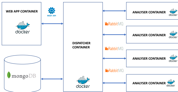
Figure 2: OpenSZZ, Web Application Architecture
