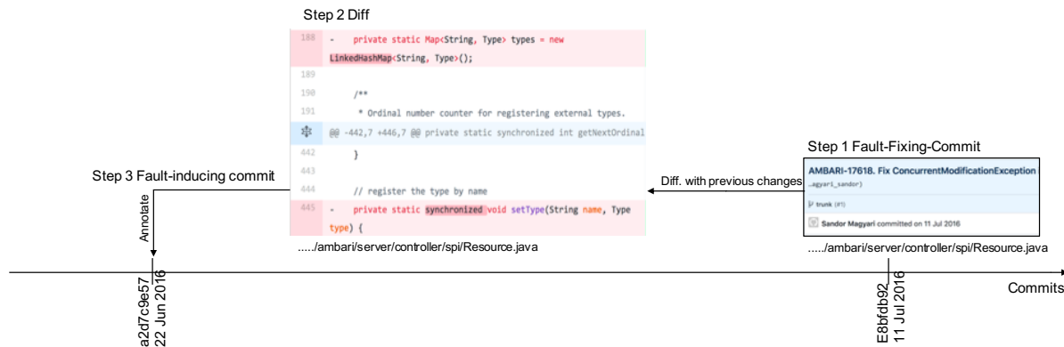
Figure 1: The OpenSZZ Approach, an outline.
