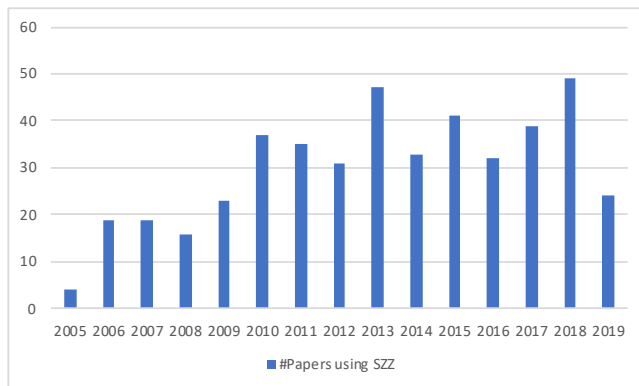
Figure 4: Number of papers using the SZZ [24] algorithm
