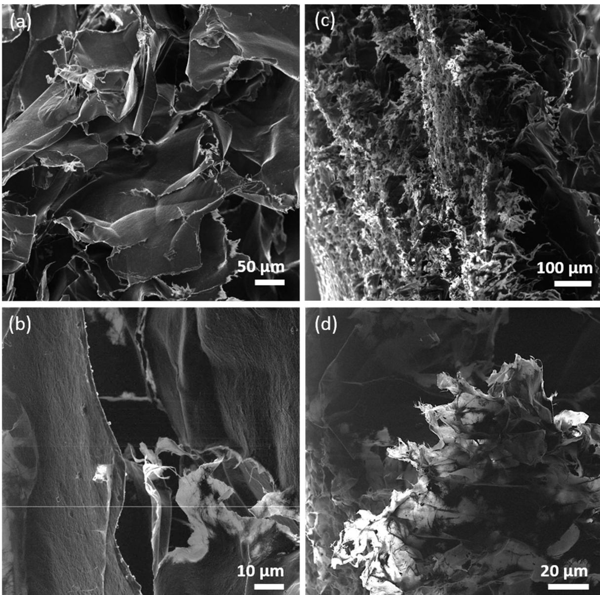
Fig. 2. Scanning helium ion microscope (HIM) images of (a-b) CNF and (c-d) CNC aerogels.
