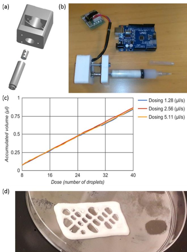
Fig. 3. (a) CAD drawing of dispenser building blocks, and (b) photograph of the nanocellulose filled syringe assembled into the dispenser system. (c) Accumulated volumes of CNF dispersion using volume of 25ul with different dosing rates. (d) An example of 3D-printed CNF-gel structure.
