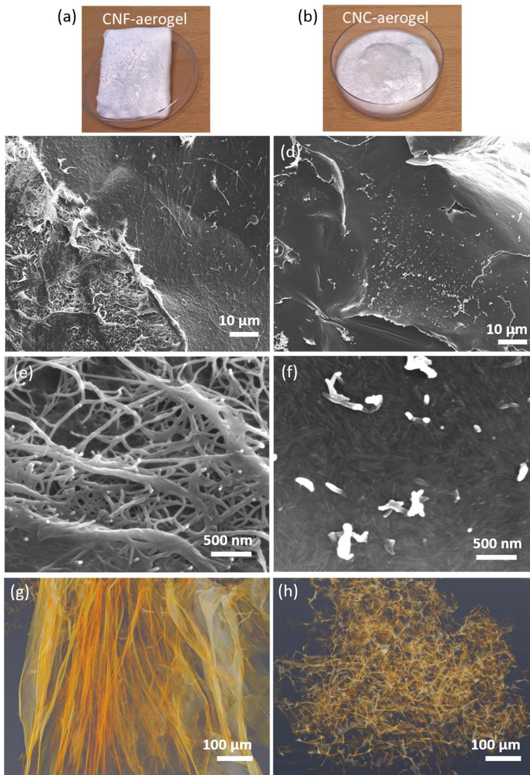
Fig. 1. Photographs of (a) CNF and (b) CNC aerogels. Scanning electron microscope (SEM) images of the (c, e) CNF and (d, f) CNC aerogels surfaces. \mu CT (X-ray micro-computed tomography) images of (g) CNF and (h) CNC aerogels.
