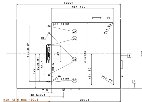
Fig. 4. Process module interface. Top view.
