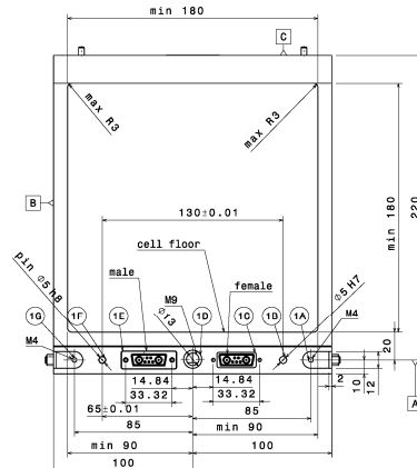
Fig. 3. Cell-to-cell interface. View at front.
