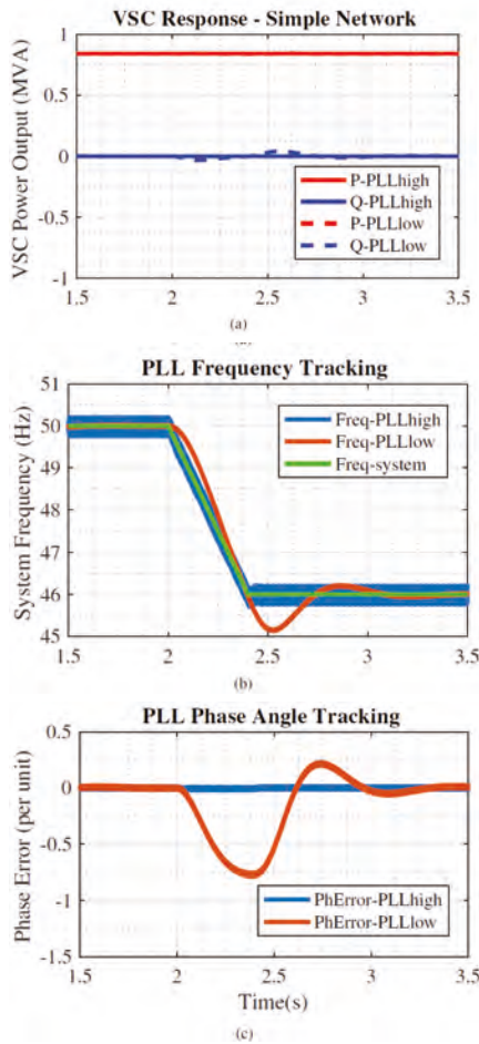
Figure 8. Simulation results with a simplified network and different PLL parameters (see Table 1)—(a) VSC output (b) PLL frequency tracking (c) PLL phase angle tracking.
