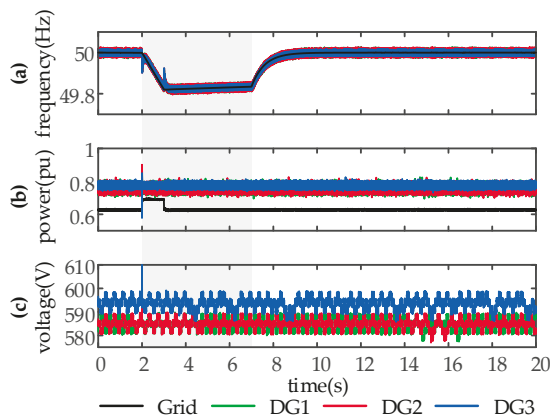
Figure 10. Responses to a short circuit fault when conventional PV systems are applied as DG1–DG3: (a) Frequency response; (b) output active power; (c) dc link voltage of the inverter.
