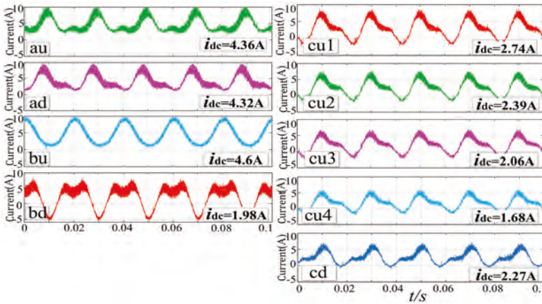
Figure 18. The currents of the battery modules.
