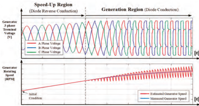
Figure 3. Waveforms of 3-phase generator voltages by diode rectifier and estimated speed using conventional SRF-PLL method.
