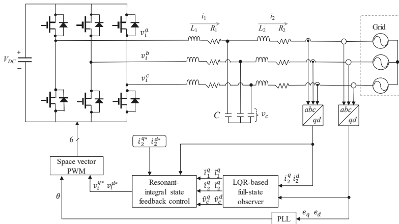
Figure 2. Block diagram of the proposed integral-resonant state feedback current control scheme with observer.
