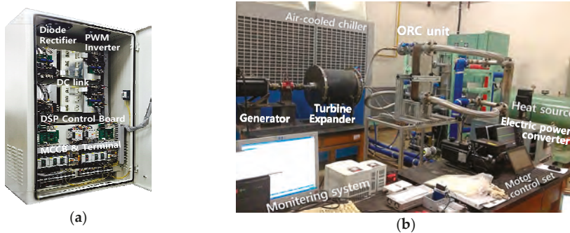
Figure 10. Experimental setup for the actual ORC power generation system: (a) Grid-connected electric power conversion system; and (b) 23 kW ORC power generation system.
