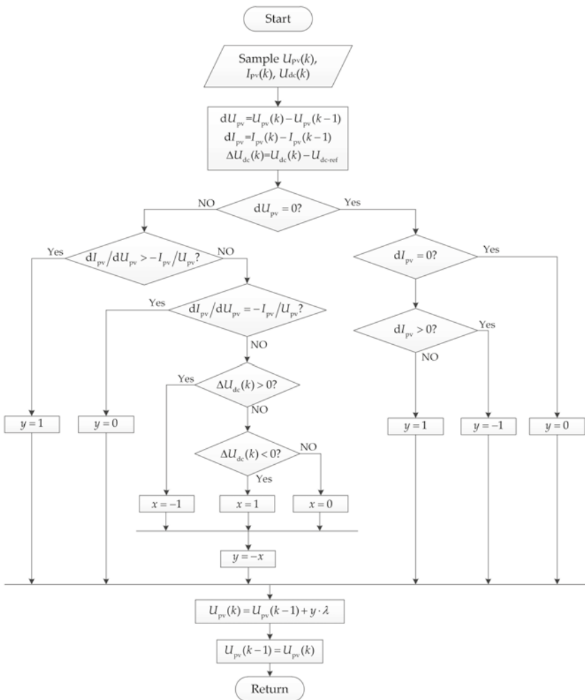
Figure 6. Adaptive-MPPT algorithm.
