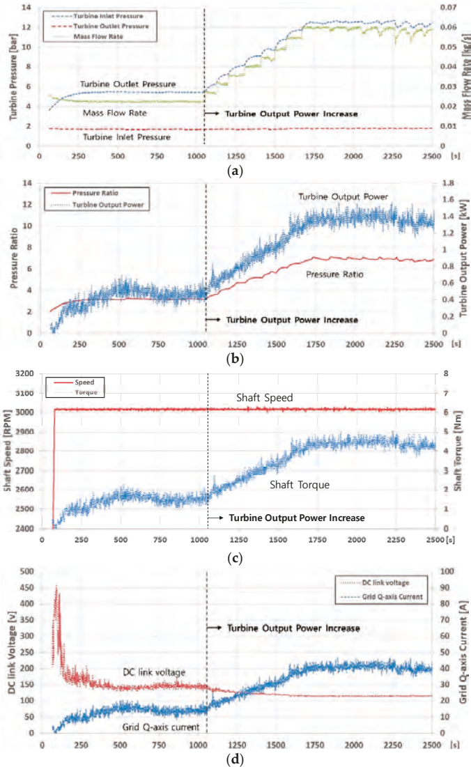
Figure 11. Experimental results of proposed speed control in the actual ORC generation system: (a) Mass flow rate of working fluid and turbine in/outlet pressure; (b) pressure ratio and turbine output power; (c) Rotation speed and torque of the turbine-generator; and (d) DC-link voltage and grid-side torque component (q-axis) current.
