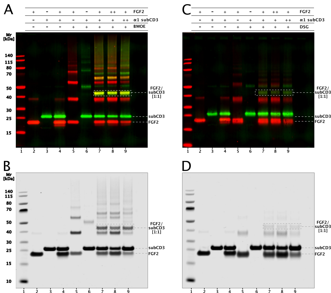
Fig. 3 The basic binding unit between FGF2 and \alpha 1 -subCD3 is a heterodimer as analyzed by chemical crosslinking experiments. FGF2 and \alpha 1 -subCD3 were mixed at a total concentration of 20 \mu M at molar ratios of 1:1 (+/+), 1:2 (+/++), and 2:1 (+/+/+) (FGF2/ \alpha 1 -subCD3). As chemical crosslinkers, bismaleidomethane (BMOE) and disuccinimidyl glutarate (DSG) were used at the molar ratios provided in Methods. Samples were analyzed by SDS-PAGE followed by either western blotting ( a , c ) or total protein staining using Coomassie. FGF2 and \alpha 1 -subCD3 migrate with an apparent molecular weight of 18 and 27 kDa, respectively. The crosslinking product with an apparent stoichiometry of 1:1 shows a migration behavior that corresponds to a molecular weight of about 45 kDa as indicated. Lane 1: molecular weight standards; lane 2: input FGF2; lane 3: input \alpha 1 -subCD3; lane 4: FGF2 plus \alpha 1 -subCD3 without crosslinker; lane 5: FGF2 plus crosslinker; lane 6: \alpha 1 -subCD3 plus crosslinker; lanes 7–9: FGF2 plus \alpha 1 -subCD3 at 1:1, 2:1, and 1:2 stoichiometries in the presence of crosslinker. a BMOE: immunoblots using anti-FGF2 and anti- \alpha 1 primary antibodies. c DSG: immunoblots using anti-FGF2 and anti- \alpha 1 primary antibodies. b BMOE: total protein visualized by Coomassie staining. d DSG: total protein visualized by Coomassie staining.
