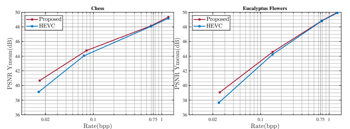
Fig. 5. Rate-distortion analysis between the proposed compression scheme and the HEVC scheme for 5 \times 5 key views.
