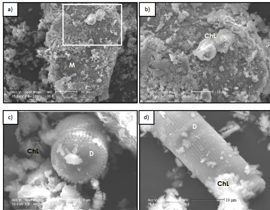
Figure 4. Micrographs of Perniö clay ( z = 4.5 m).
