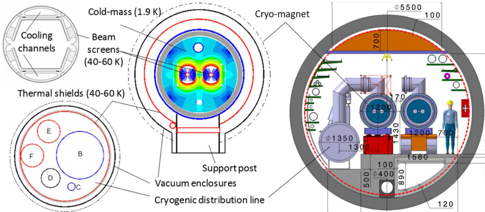
Fig. 5.12. Cross-section of the tunnel and main cryogenic components.
