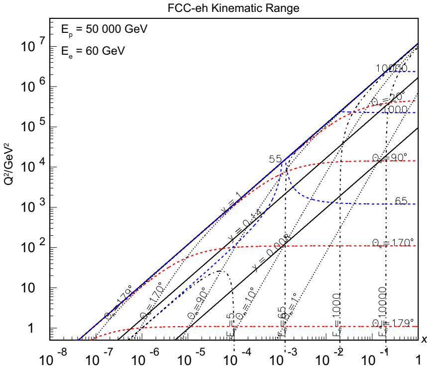
Fig. 7.27. Kinematics of the FCC-eh for E_p = 50 TeV and E_e = 60 GeV. Blue dashed lines: constant scattered electron energy, which for Q^2 below 1000 GeV 2 never exceeds 65 GeV. Red dashed lines: constant electron polar angle. One observes that the low x region is very accessible with a detector acceptance down to one degree for backward electrons. Black dashed-dotted lines: constant hadronic final state energy. At large Bjorken x , energies of up to tens of TeV are scattered in the forward detector region; black dotted lines: constant polar angle of the hadronic final state.
