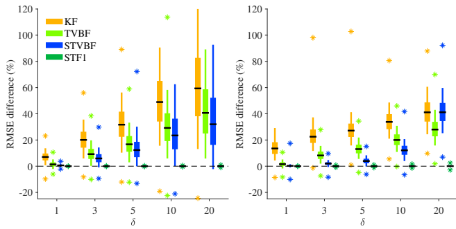
Fig. 8. The proposed STF outperforms the comparison methods with skew- t -distributed noise. RMSE differences from STF's RMSE per cent of the STF's RMSE. The difference to STVBF [20] increases as skewness increases or when process noise variance reduces. (left) q = 0.5 , (right) q = 5 .
