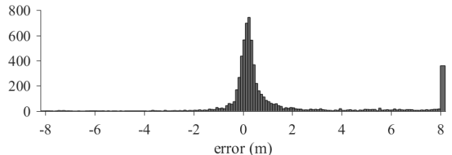
Fig. 1. The error histogram in an ultra-wideband (UWB) ranging experiment described in [8] shows positive skewness. The edge bars show the errors outside the figure limits.
