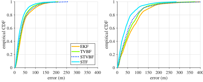
Fig. 12. Empirical error CDFs for the real GNSS data for the horizontal error (left) and the vertical error (right)
