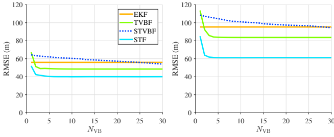
Fig. 11. RMSE of horizontal (left) and vertical (right) position for real GNSS data as a function of the number of VB iterations
