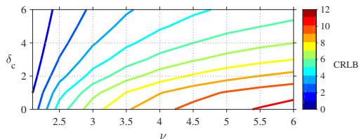
Fig. 14. The CRLB of the 50th time instant for the model (43) with a fixed measurement noise variance. Skewness and heavy-tailedness decreases the CRLB significantly.
