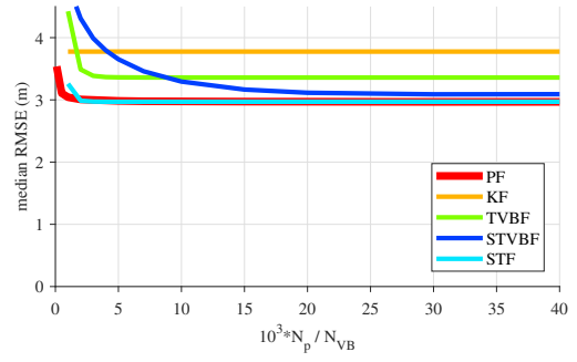
Fig. 7. The proposed STF's median RMSE does not improve after N_{VB}=5 VB iterations per time instant. The required number of PF particles N_p can be more than 10000, and STVBF [20] can require 30 VB iterations. The x -axis is 10^3 \cdot N_p for PF and N_{VB} for the rest of the filters. q=5 , \delta=5 .
