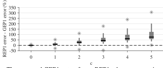
Fig. 5. The proposed GEP1 outperforms REPI when one negative outlier is added to the measurement noise vector because there is one truncation that truncates much more probability than the rest.
