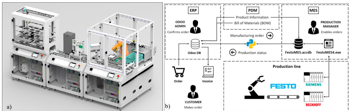
Fig.1. (a) Manufacturing line of the cyber-physical system's laboratory; (b) PDM, ERP and MES integration to the manufacturing line.
