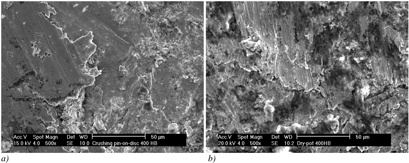
Figure 8. Scanning electron microscope images of the wear surfaces of the 400 HB grade steel samples tested with a) crushing pin-on-disc, and b) dry-pot.
