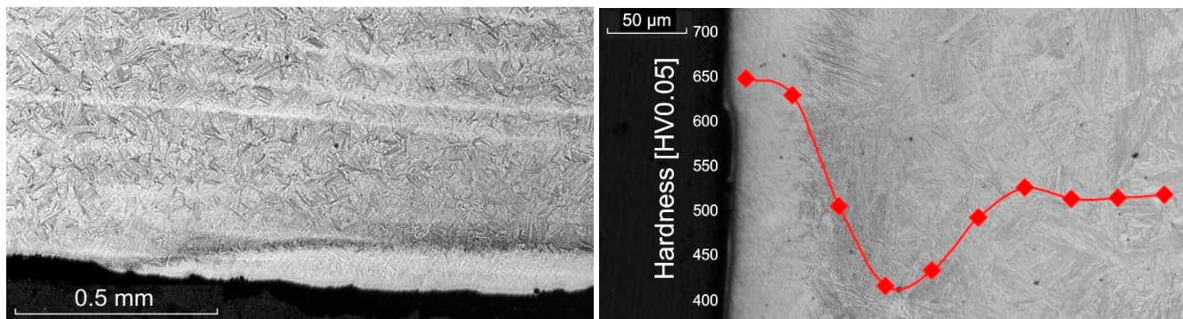
a) b) Figure 4. Optical micrograph of the underside cross-section of the cutting edge showing a) a white layer and b) a typical hardness profile over a white layer.
