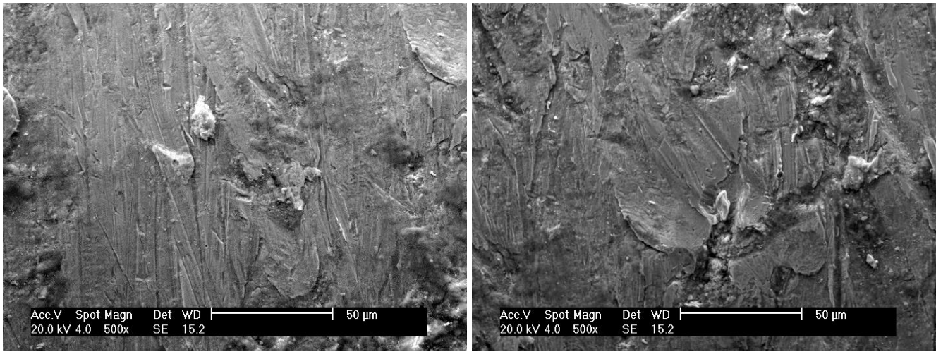
c) d) Figure 3. Scanning electron microscope images of the cutting edge wear surfaces a) top part, b) tip on the underside, and c), d) underside. The arrow indicates a crack.
