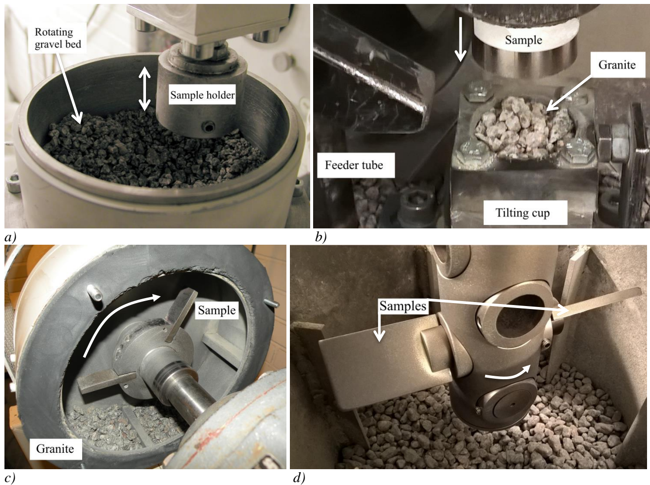
Figure 2. Test chambers of the used wear testing devices with samples: a) crushing pin-on-disc, b) uniaxial crusher, c) impeller-tumbler, and d) dry-pot.
