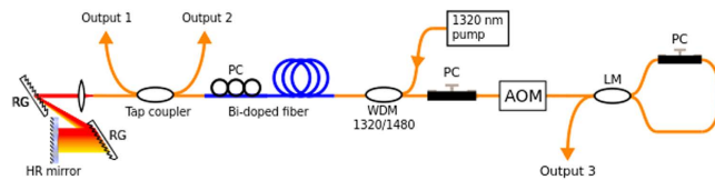
Figure 1. Bi-doped FSF fibre laser setup. AOM – acousto-optic modulator, WDM – wavelength division multiplexer, PC – polarization controller, LM – loop mirror, RG – reflection grating, HR mirror – high reflective mirror.
