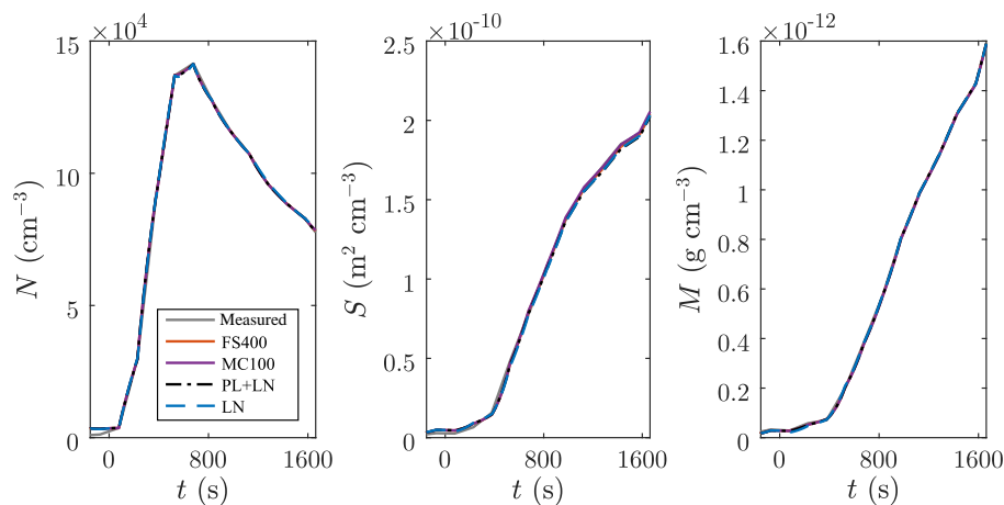
Figure 5. Number ( N ), surface area ( S ), and mass ( M ) concentrations of the nucleation mode in the chamber event. The measured concentrations and the concentrations produced during inverse modeling using different models are nearly equal. The data are shown for the centers of the Nano-SMPS scans only, because those values only are used in inverse modeling. FS400 denotes the fixed-sectional model with 400 size sections and MC100 denotes the moving-center fixed-sectional model with 100 size sections.
