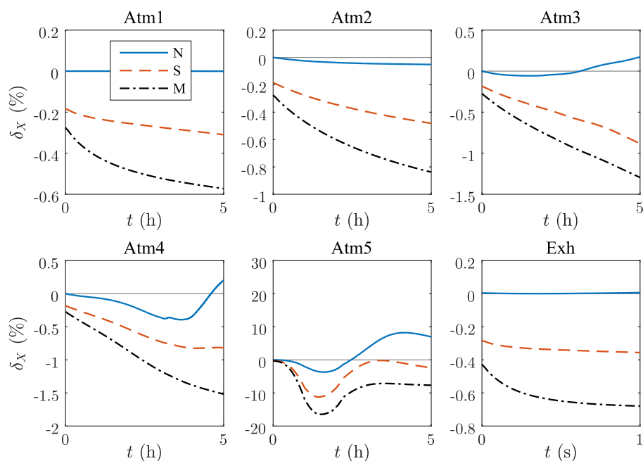
Figure 10. The relative errors of the moments ( \delta_X ) in the test cases produced by the PL+LN model. The input parameter sets are shown in Table 1.
