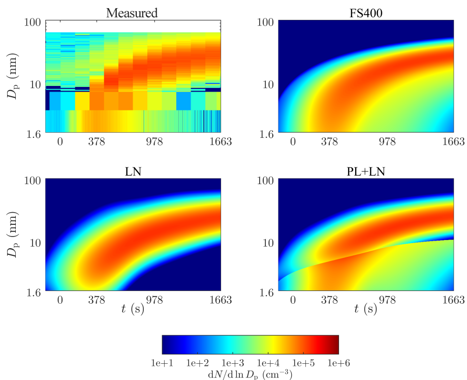
Figure 11. Contour plots of particle distributions measured by the Airmodus Particle Size Magnifier (PSM), TSI Ultrafine Condensation Particle Counter (CPC), and TSI Nano Scanning Mobility Particle Sizer (Nano-SMPS) and simulated by different models in the chamber event. The value of 0.8 was used for \gamma with the PL+LN model. The UV lights were switched on at time t = 0 s. Note that the background particle distribution seen in the measured data was excluded from the simulations.
