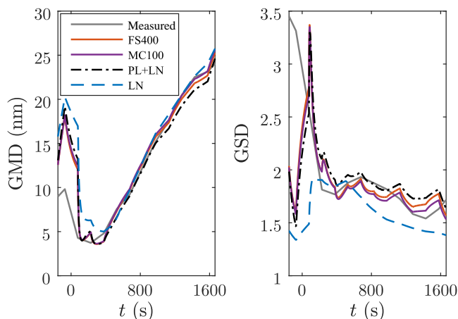
Figure 8. Geometric mean diameter (GMD) and geometric standard deviation (GSD) of the nucleation mode in the chamber event, obtained through inverse modeling, using different models.
