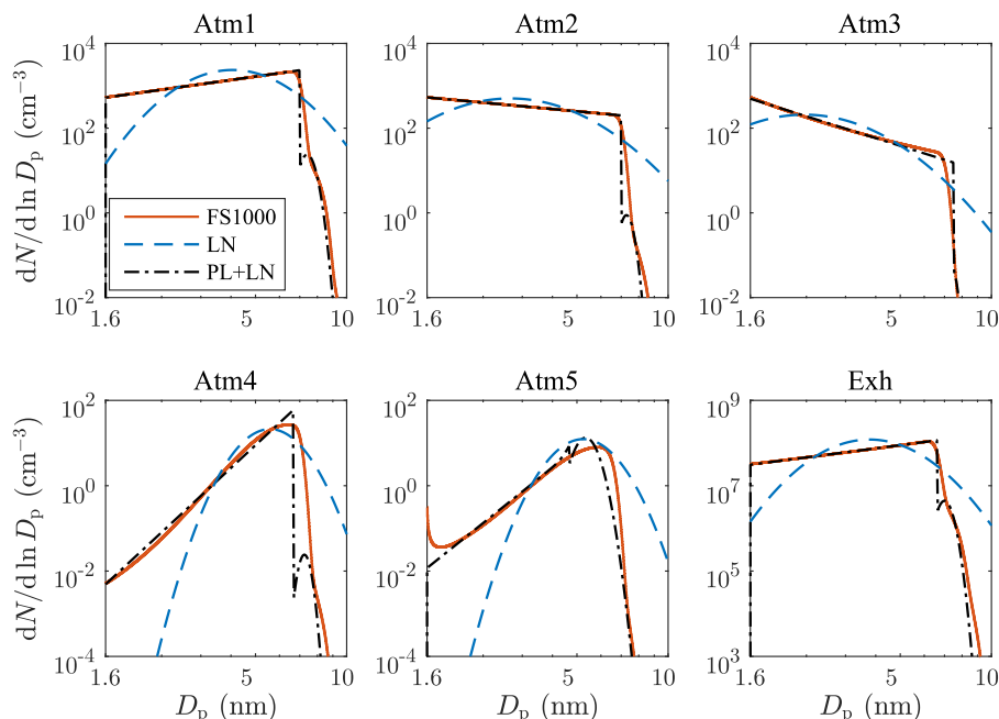
Figure 9. Particle size distributions at the ends of the test case simulations produced by different models. The input parameter sets are shown in Table 1. FS1000 denotes the fixed-sectional model with 1000 size sections. Note the different scales in the vertical axes on the bottom row.
