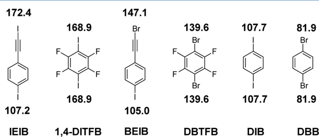
Figure 19. Chemical structures of C(sp)-bonded XB donors (IEIB and BEIB), activated C(sp 2 )-bonded donors (1,4-DITFB and DBTFB), and nonactivated C(sp 2 )-bonded donors (DIB and DBB) cocrystallized using a solvent-drop grinding methodology. The six XB donor molecules are reported in order of decreasing V_{S,max} values (from left to right) associated with the most positive \sigma -hole on their halogen atoms. V_{S,max} values are the numbers reported near the corresponding atom and are given in kilojoules per mole. Adapted with permission from ref 209. Copyright 2013 John Wiley and Sons.
