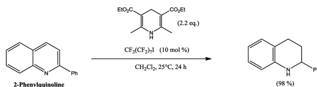
Figure 123. Reduction of 2-phenylquinoline in the presence of 1-iodoperfluorooctane.
