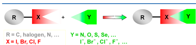
Figure 1. Schematic representation of the halogen bond.
