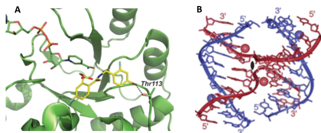
Figure 113. (A) XB (dotted black line) between the Br of IDD594 and the O( \gamma ) of Thr113 in human aldose reductase. (B) Atomic structure of d(CCAGTACBr 5 UGG), with bromine atoms rendered as spheres and the deoxyribose backbones as solid ribbons. Panel A reprinted with permission from ref 27. Copyright 2011 Royal Society of Chemistry. Panel B reprinted from ref 878. Copyright 2003 American Chemical Society.
