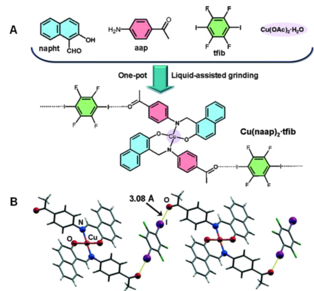
Figure 101. (A) Molecular structures of single compounds (top) employed in LAG synthesis of a halogen-bonded MOF (bottom). (B) Partial representation of the crystal structure resulting from a combination of covalent bond formation, coordination bonds, and XBs. I...O XBs are shown as yellow solid lines, and the I...O distance is reported ( N_c = 0.88 ). Adapted with permission from ref 801. Copyright 2014 Royal Society of Chemistry.
