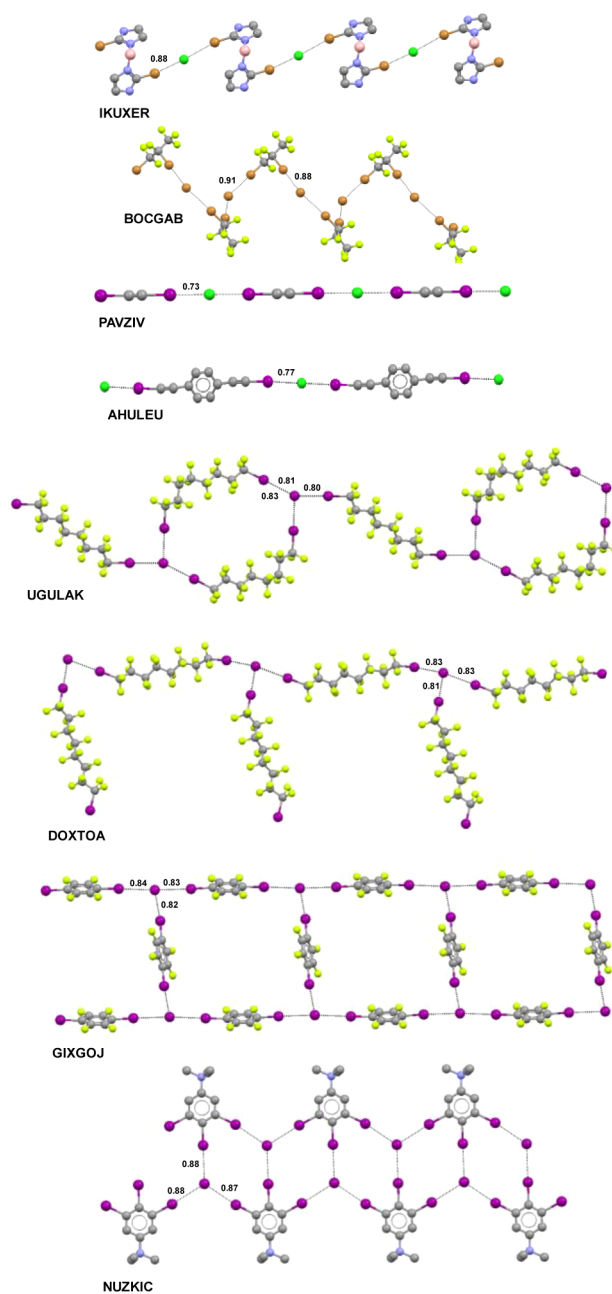
Figure 77. Infinite chains produced on C-Br \cdots Cl^- XB formation in bis(2-bromoimidazole)boronium chloride (IKUXER), 742 C-Br \cdots Br^- XB formation in (-)-sparteine hydrobromide/1,2-dibromohexafluoropropane (BOCGAB), 263 C-I \cdots Cl^- XB formation in bis[bis(ethylenedithio)tetrathiafulvalene] chloride/diiodoacetylene (PAVZIV), 665 and C-I \cdots Cl^- XB formation in tris[bis(ethylenedithio)tetraselenafulvalene] chloride/1,4-bis(iodoethynyl)benzene (AHULEU). 743 Cations and hydrogen atoms are omitted for simplicity. "Rings and sticks" (UGULAK) and comblike (DOXTOA) architectures form when iodide anions (tridentate nodes) self-assemble with \alpha,\omega -diiodoperfluoroalkanes. Halogen-bonded ribbons form when iodide anions (tridentate nodes) self-assemble with 1,4-DITFB (GIXGOJ), 75 or with a triiodobenzene derivative (NUZKIC). 744 Color code: carbon, gray; nitrogen, blue; iodine, purple; chlorine, light green; boron, pink; fluorine, yellow. XBs are dotted black lines. CSD Refcodes are reported.
