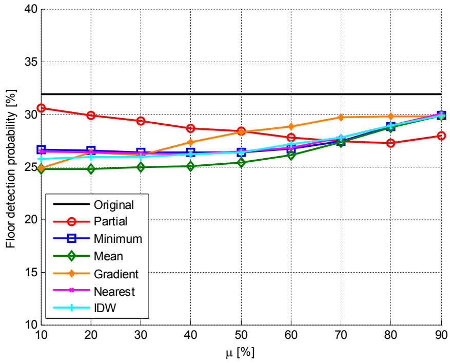
Figure 21. Mean floor detection probability as a function of \mu considering all user tracks for original fingerprints, partial fingerprints (after removal process) and for different extrapolation methods after interpolation at 5GHz band
