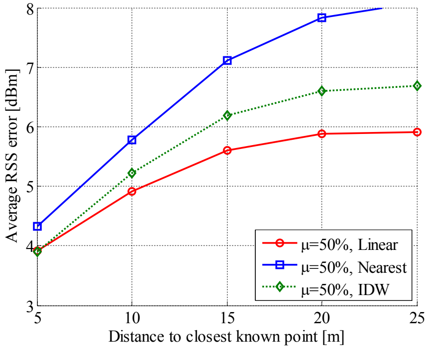
Figure 10. Average interpolation RSS error as a function of distance to the closest known fingerprint at 2.4GHz band
