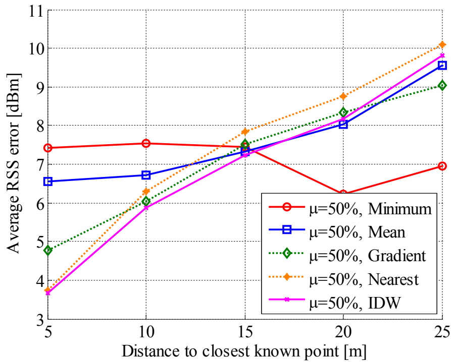
Figure 11. Average extrapolation RSS error as a function of distance to the closest known fingerprint at 2.4GHz band
