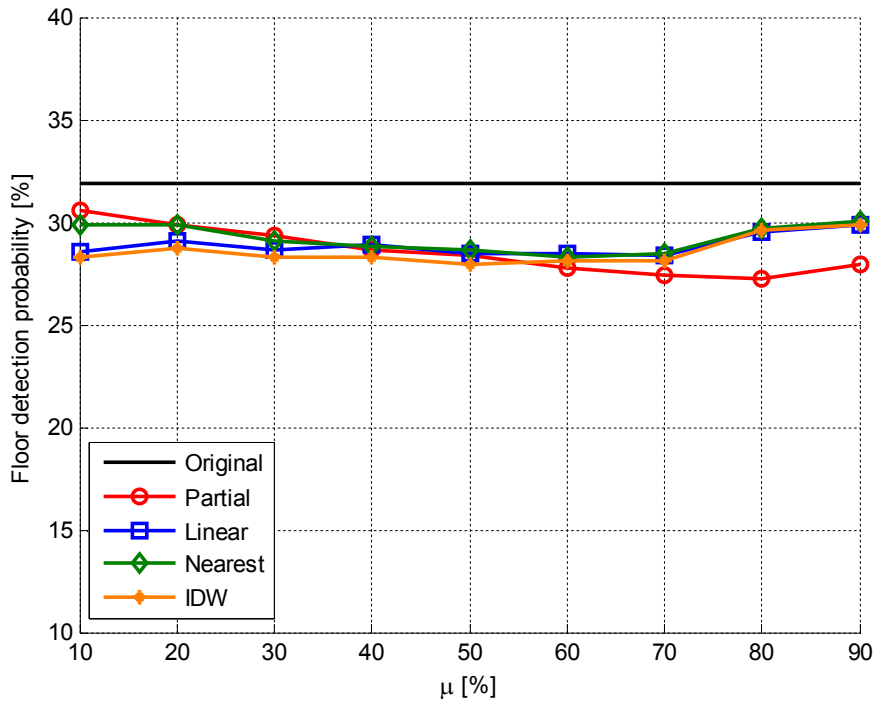
Figure 19. Mean floor detection probability as a function of \mu considering all user tracks for original fingerprints, partial fingerprints (after removal process) and for different interpolation methods at 5GHz band
