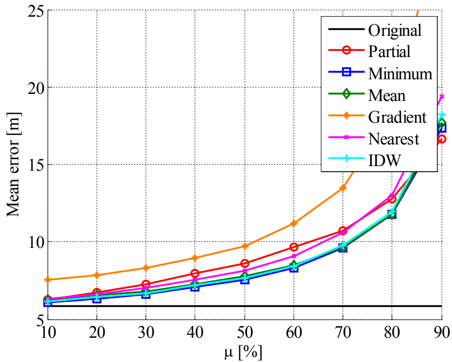
Figure 14. Mean positioning error as a function of \mu considering all user tracks for original fingerprints, partial fingerprints (after removal process) and for different extrapolation methods after interpolation at 2.4GHz band
