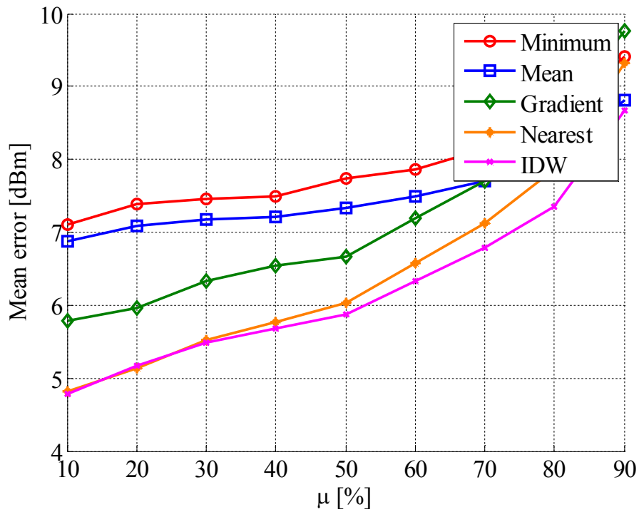
Figure 7. Mean error of extrapolated RSS values as a function of fingerprint removal percentage \mu at 2.4GHz band
