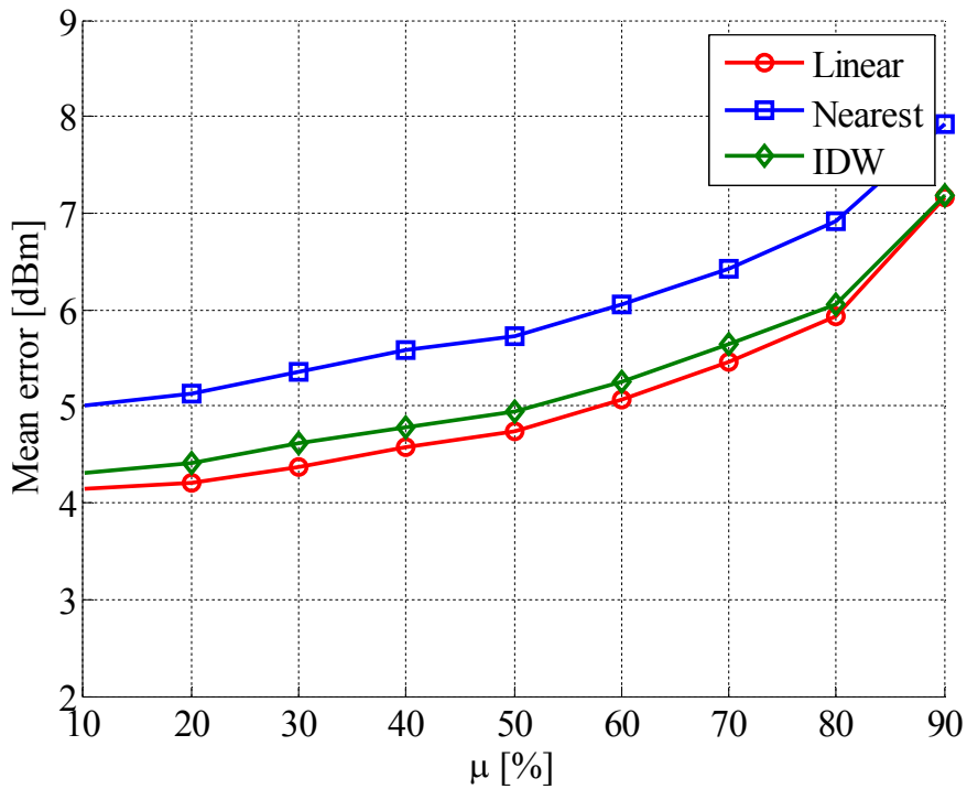
Figure 6. Mean error of interpolated RSS values as a function of fingerprint removal percentage \mu at 2.4GHz band
