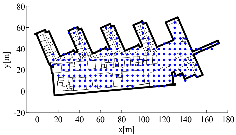
Figure 2. Original full fingerprint database ( \Omega_{full} ) with g_{int}=5m for the first floor at 2.4GHz band
