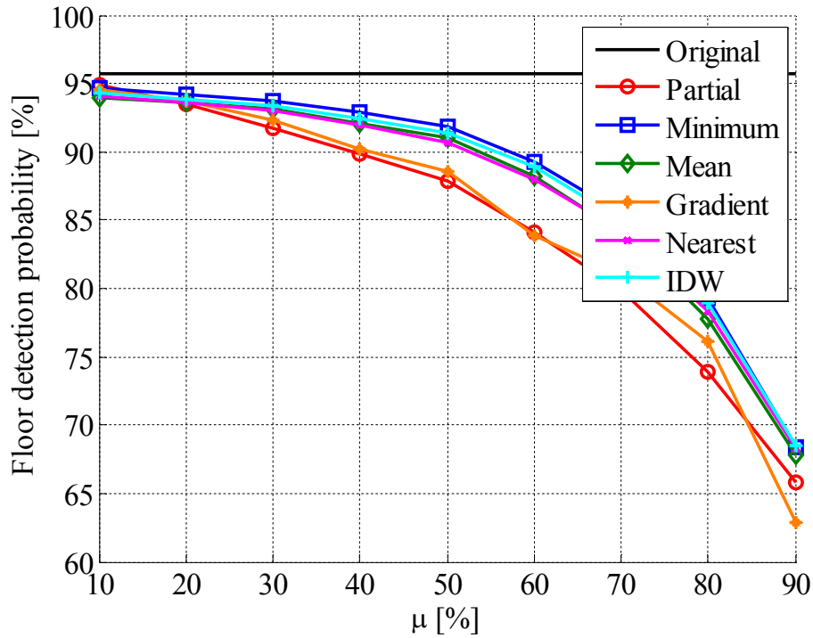
Figure 15. Mean floor detection probability as a function of \mu considering all user tracks for original fingerprints, partial fingerprints (after removal process) and for different extrapolation methods after interpolation at 2.4GHz band
