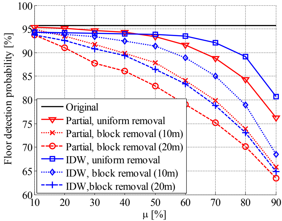
Figure 17. Mean floor detection probability as function of \mu considering all user tracks for original fingerprints, partial fingerprints and IDW interpolated and extrapolated fingerprints for uniform fingerprint removal, and block removal with d_{block}=10m and d_{block}=20m at 2.4GHz band
