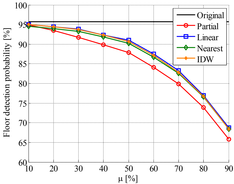
Figure 13. Mean floor detection probability as a function of \mu considering all user tracks for original fingerprints, partial fingerprints (after removal process) and for different interpolation methods at 2.4GHz band
