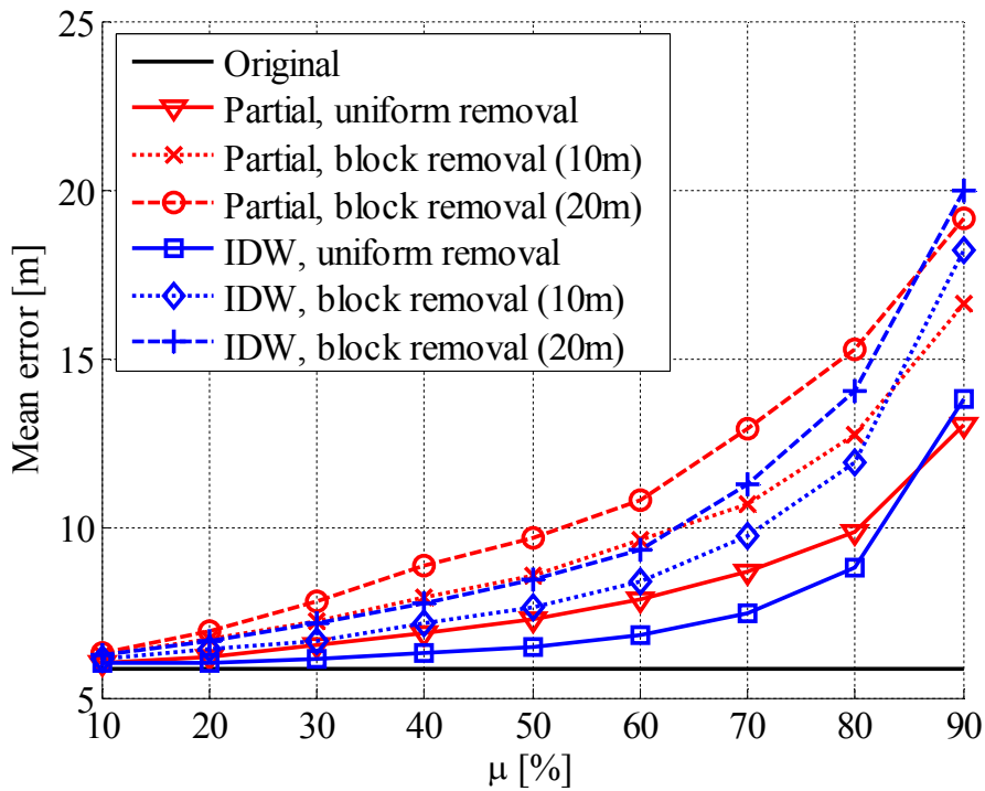
Figure 16. Mean positioning error as function of \mu considering all user tracks for original fingerprints, partial fingerprints and IDW interpolated and extrapolated fingerprints for uniform fingerprint removal, and block removal with d_{block}=10m and d_{block}=20m at 2.4GHz band
