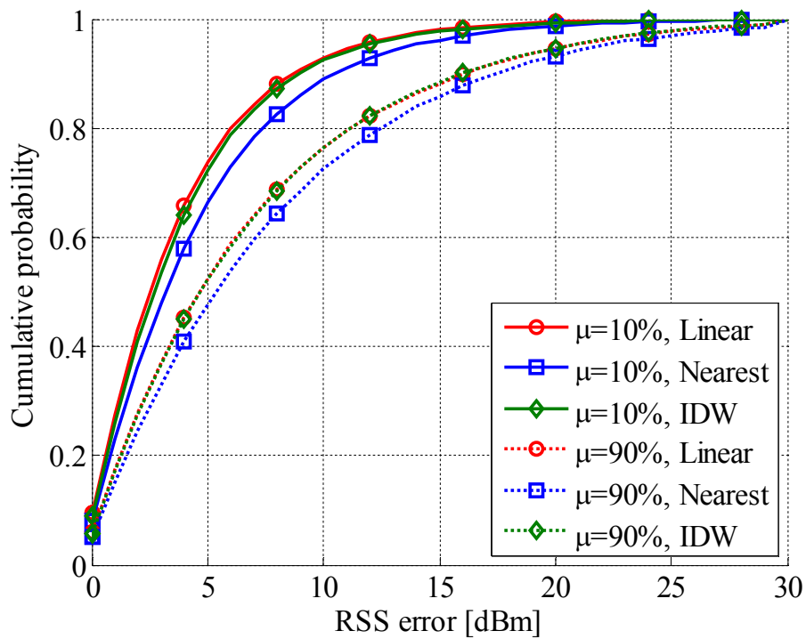
Figure 8. Cumulative error distribution of interpolated RSS values at 2.4GHz band
