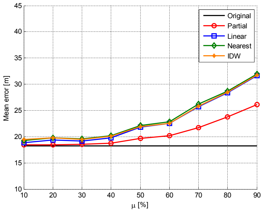
Figure 18. Mean positioning error as a function of \mu considering all user tracks for original fingerprints, partial fingerprints (after removal process) and for different interpolation methods at 5GHz band
