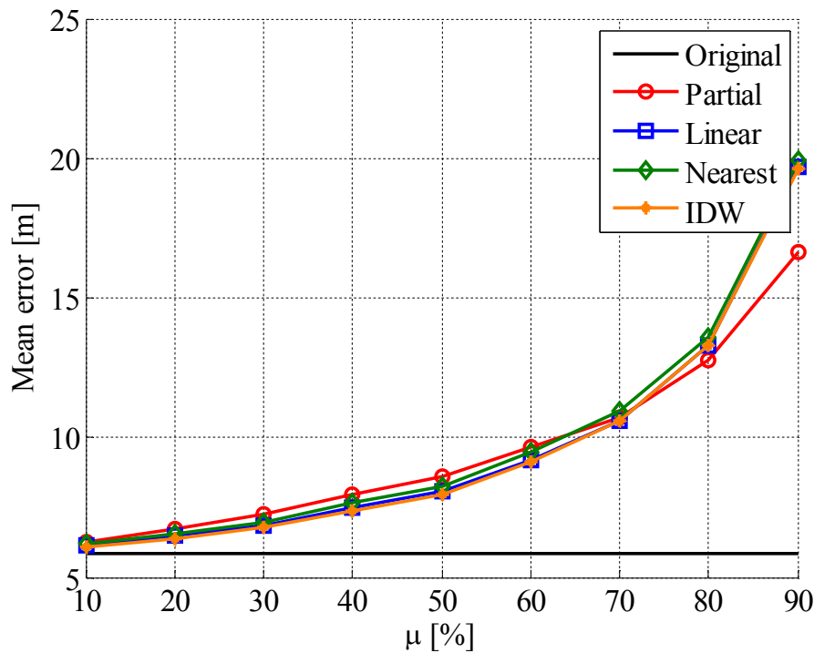
Figure 12. Mean positioning error as a function of \mu considering all user tracks for original fingerprints, partial fingerprints (after removal process) and for different interpolation methods at 2.4GHz band
