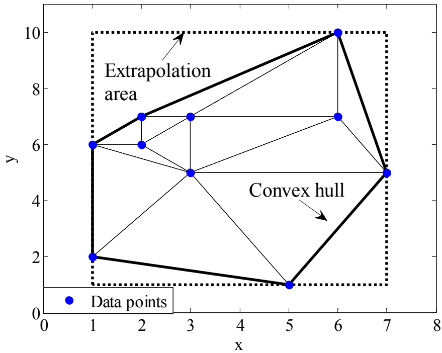
Figure 4. Illustration of interpolation and extrapolation areas and the considered Delaunay triangulation for data points (fingerprints) originated from one imaginary AP in one floor
