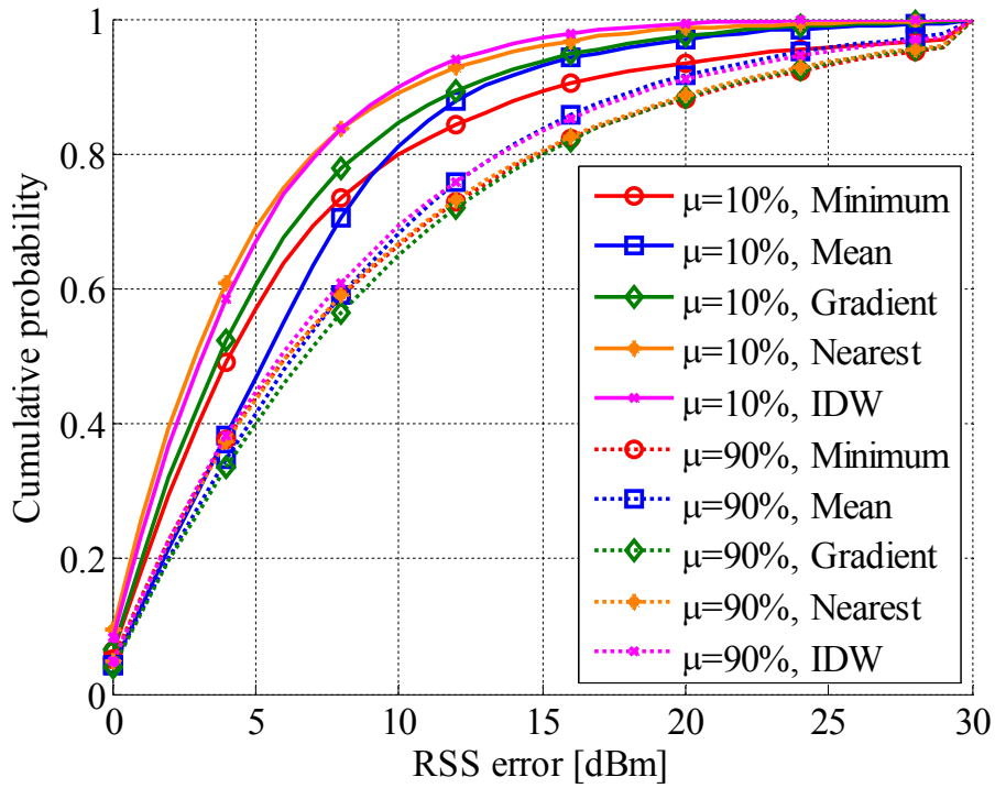
Figure 9. Cumulative error distribution of extrapolated RSS values at 2.4GHz band
