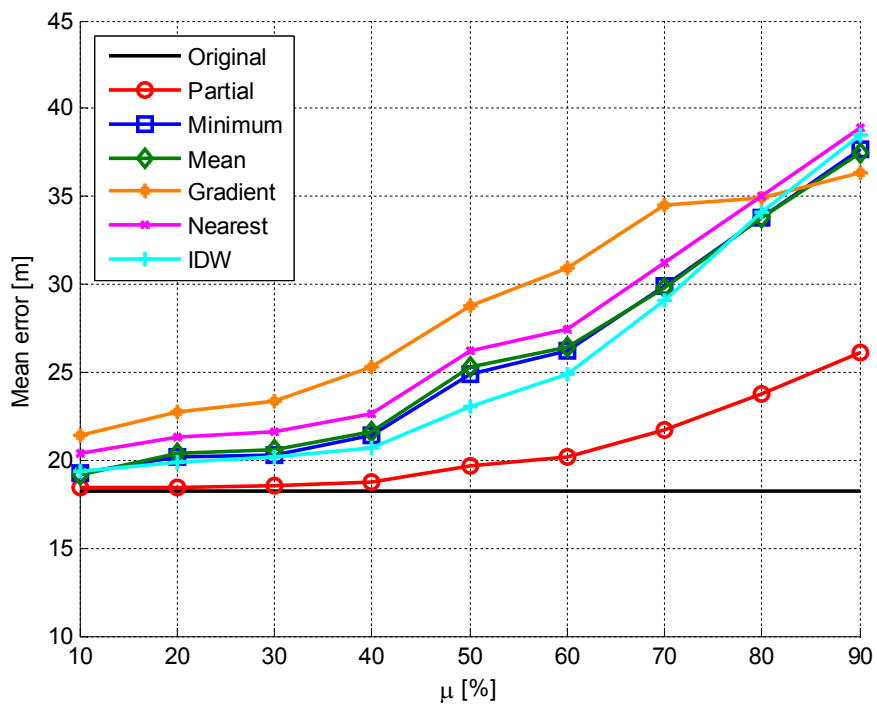
Figure 20. Mean positioning error as a function of \mu considering all user tracks for original fingerprints, partial fingerprints (after removal process) and for different extrapolation methods after interpolation at 5GHz band
