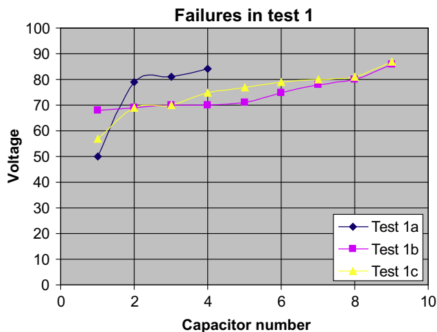
Fig. 3. Failure voltages in test 1.
