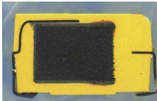
Fig. 5. A cross-section of a failed capacitor.
