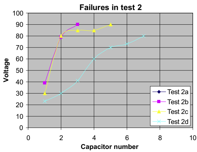
Fig. 4. Failure voltages in test 2.
