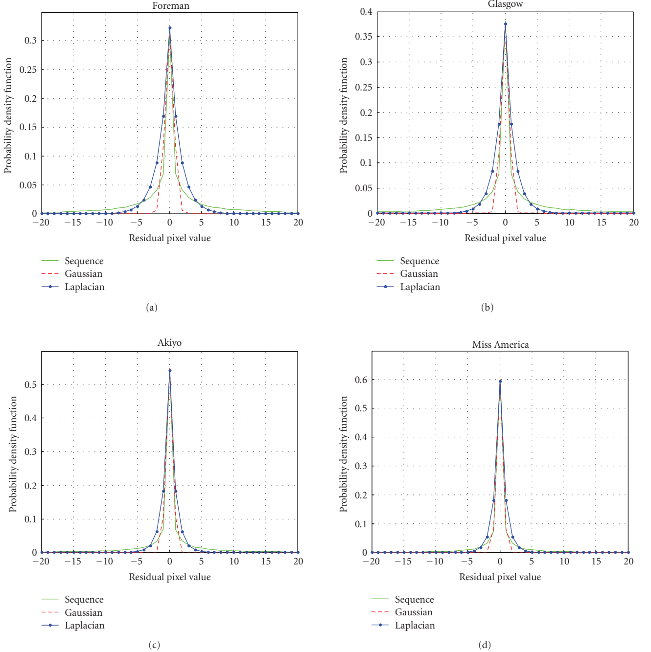
FIGURE 1: Distribution of the residual pix f'(x, y) of the four sequences: (a) Foreman, (b) Glasgow, (c) Akiyo, and (d) Miss America. The dashed red line shows the ideal Gaussian distribution having a zero mean and a variance approximate to that of the collected data.
