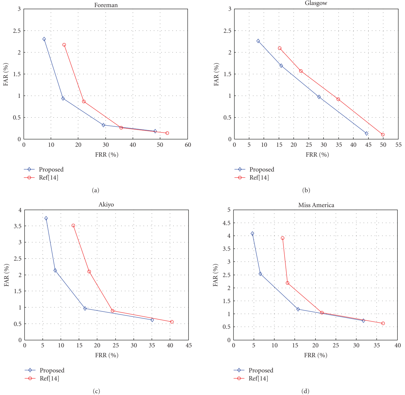
FIGURE 4: Receiver operating characteristics of the proposed method and the reference codec [14] for (a) Foreman, (b) Glasgow, (c) Akiyo, and (d) Miss America.
