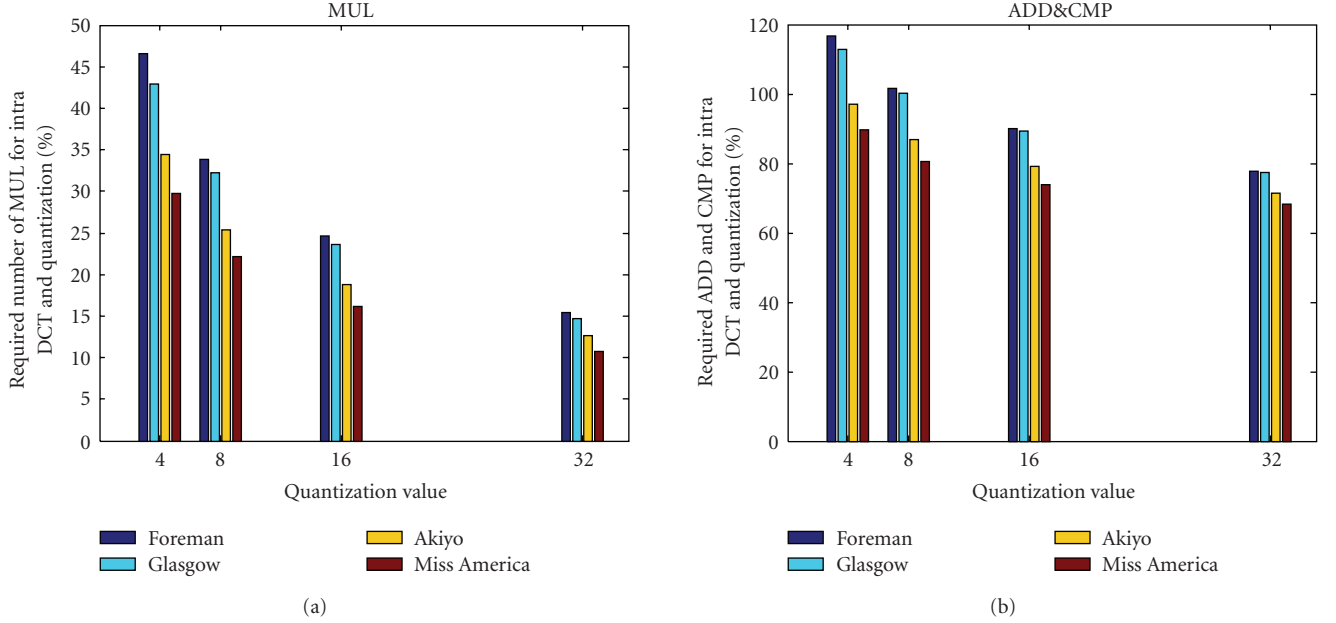
FIGURE 3: Complexity reduction for intra-DCT and quantization including the overhead computations, (a) multiplications (MULs), (b) additions (ADDs), and comparisons (CMPs).
