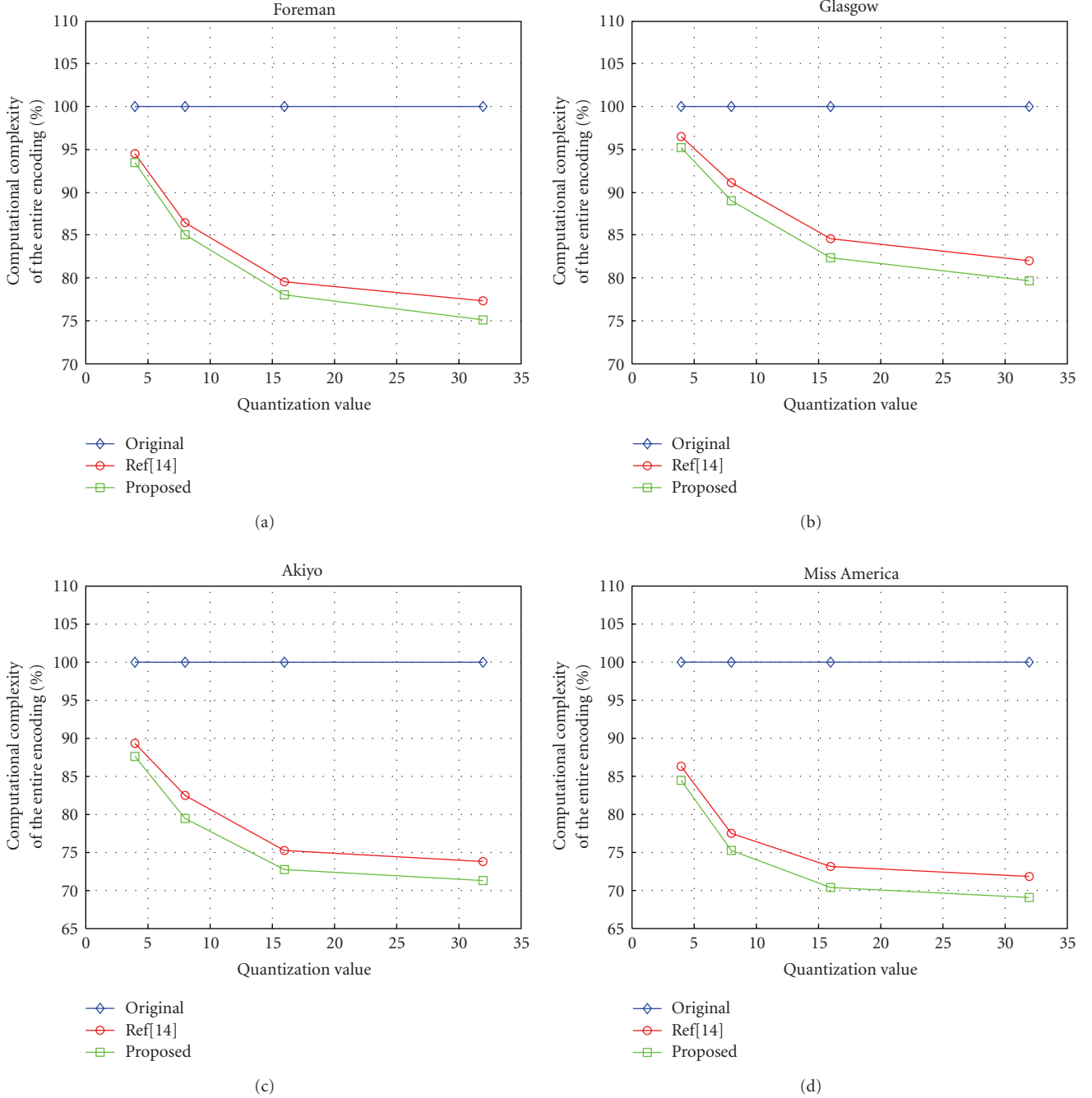
FIGURE 5: Comparison of required encoding time among the proposed hybrid model, the XIVD encoder, and the reference encoder [14] for different sequences: (a) Foreman, (b) Glasgow, (c) Akiyo, and (d) Miss America.
