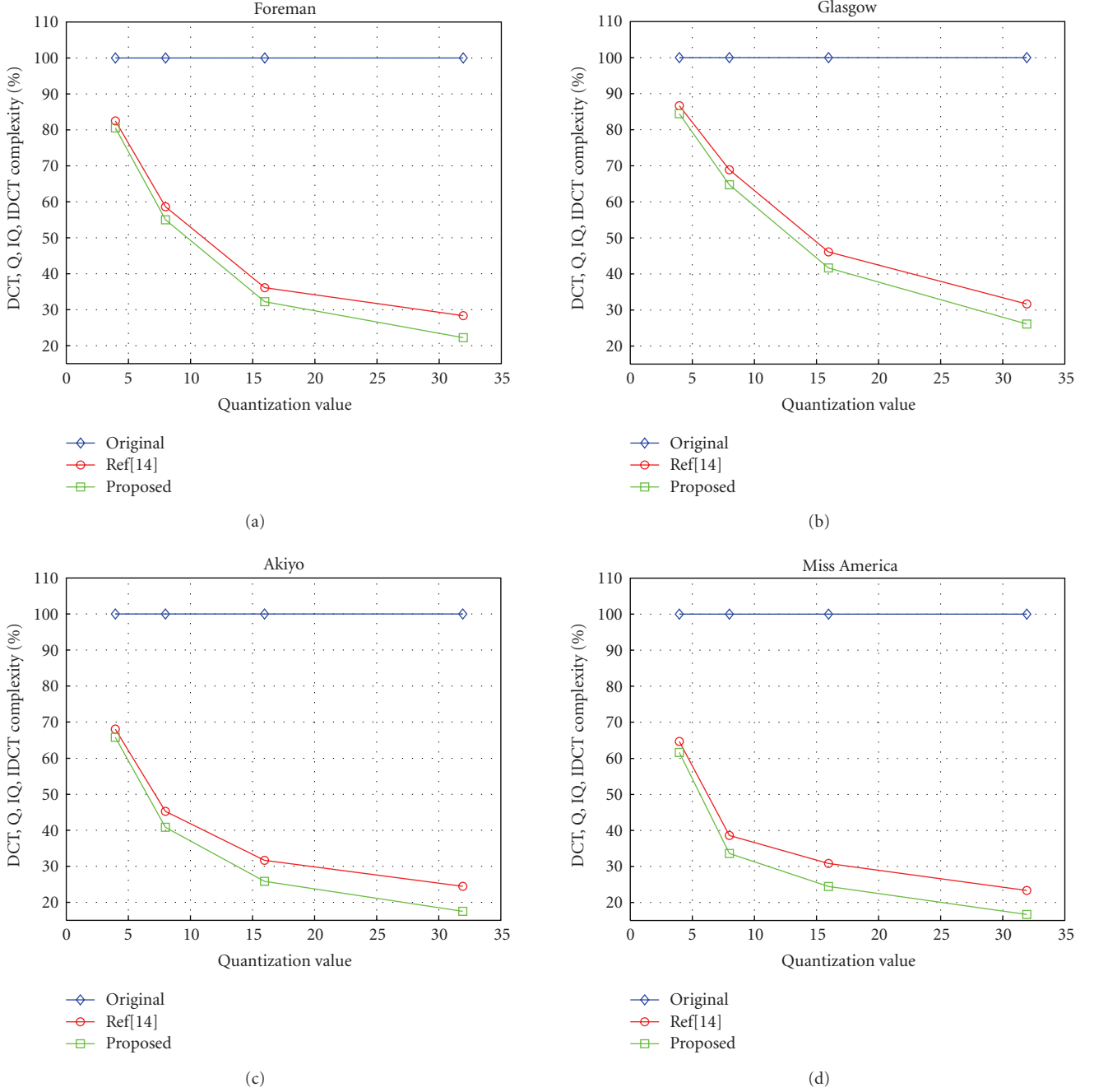
FIGURE 2: Computational reduction of the proposed model and the reference encoder [14] compared to original XVID codec for different sequences, (a) Foreman, (b) Glasgow, (c) Akiyo, and (d) Miss America.
