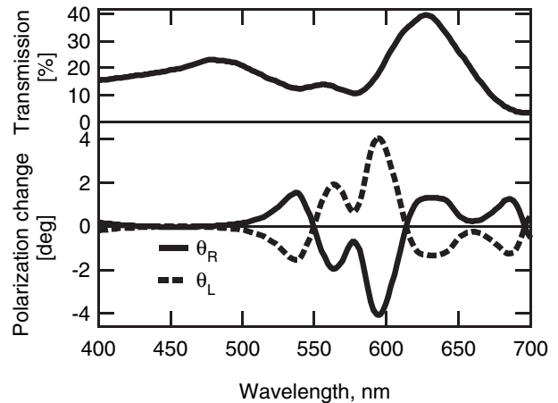
FIG. 3. Calculated transmission (top) and polarization azimuth rotation (bottom) spectra for right- and left-twisted gratings composed of 80 nm linewidth gold nanostructures of 100 nm height on the fused silica substrate. Both gratings show the same transmission but opposite polarization azimuth rotation.
