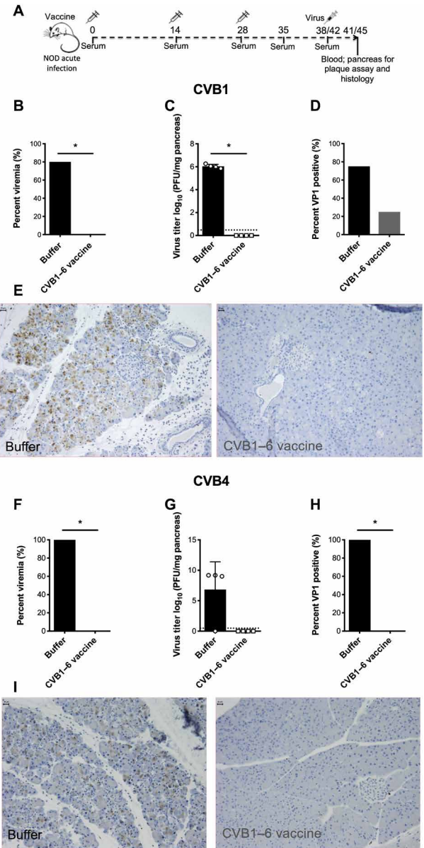
Fig. 3. CVB1–6 vaccine protects mice from acute CVB1 and CVB4 infections. Female NOD mice (4 to 6 weeks old) were mock-vaccinated (vaccine buffer; 150 \mu l, interscapularly) or CVB1–6–vaccinated (1 \mu g of each serotype, interscapularly) on days 0, 14, and 28 and then challenged with CVB1 [ 10^6 plaque-forming units (PFU) per mouse, intraperitoneally] or CVB4 ( 10^5 PFU per mouse, intraperitoneally) on days 42 and 38, respectively, as shown in the experimental schematic in (A). (B and F) Percentage of mock-vaccinated (CVB1, n = 5 ; CVB4, n = 4 ) and CVB1–6–vaccinated (CVB1, n = 4 ; CVB4, n = 4 ) mice with viremia on day 3 after infection (measured by standard plaque assay). * P < 0.05 , one-way Fisher’s exact test. (C and G) Replicating virus in the pancreas on day 3 after infection of CVB1-infected (C) or CVB4-infected (G) mice (measured by standard plaque assay). Virus titers for each mouse are shown individually. Bars represent means \pm SD. The dotted line shows the limit of detection for the assay. * P < 0.05 comparing the two groups by Mann-Whitney U test. (D and H) Percentage of pancreas sections positive for VP1 by immunohistochemical staining on day 3 after infection in CVB1-infected (D) and CVB4-infected (H) mice. * P < 0.05 , one-way Fisher’s exact test. (E and I) Representative VP1 staining in pancreas of mice infected with CVB1 (E) or CVB4 (I). Magnification, \times 16 ; scale bars, 20 \mu m. In (C) and (D), n = 4 in the buffer-treated group, as one NOD mouse was kept for longer to ensure that SOCS-1- tg animals were not single-housed.
