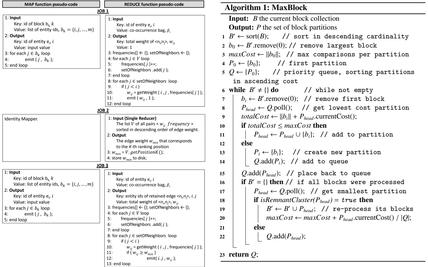
Figure 21: Pseudo-code interpretation of the entity-based strategy for CEP.
