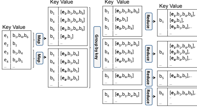
Figure 9: An example of the comparison-based strategy for Preprocessing.
