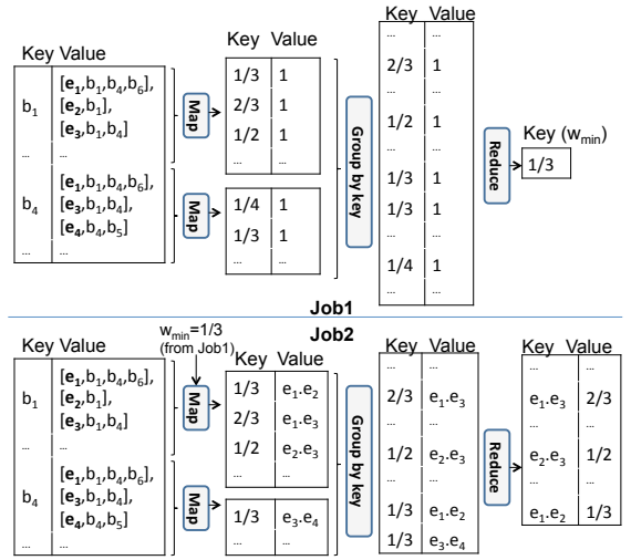
Figure 20: An example of the comparison-based strategy for CEP, using the JS weighting scheme.
