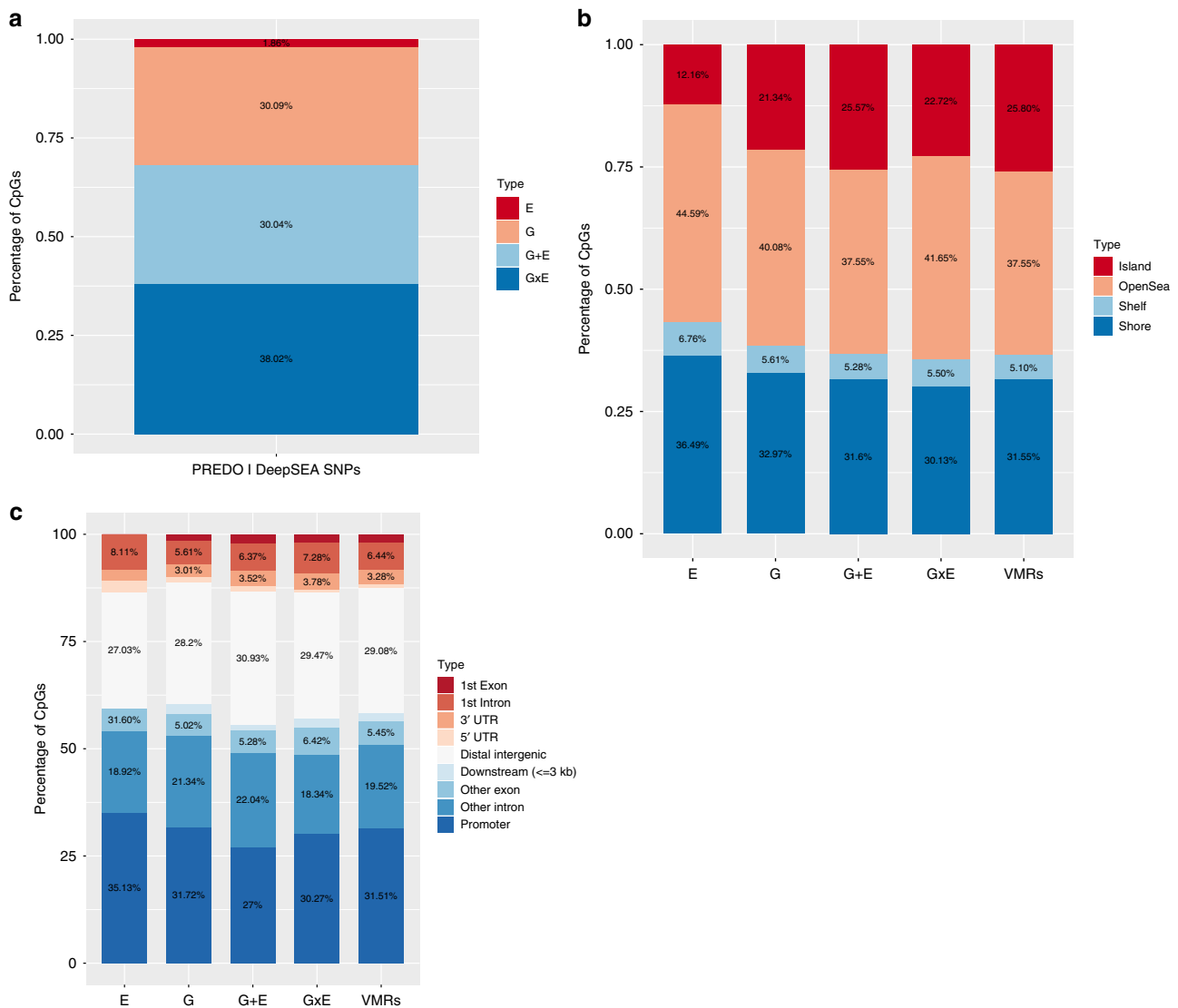
Fig. 3 VMR analysis in DeepSEA annotated SNPs in PREDO I dataset. a Percentage of models (G, E, Gx+E or G + E) with the lowest AIC explaining variable DNA methylation using the PREDO I dataset with DeepSEA annotated SNPs. b Distribution of the locations of all VMRs and tagVMRs with best model E, G, G + E and Gx+E on the 450k array using only DeepSEA variants in relationship to CpG-islands based on the Illumina 450 K annotation. c Distribution of gene-centric locations of all VMRs and tagVMRs with best model E, G, G + E and Gx+E on the 450k array using only DeepSEA variants
