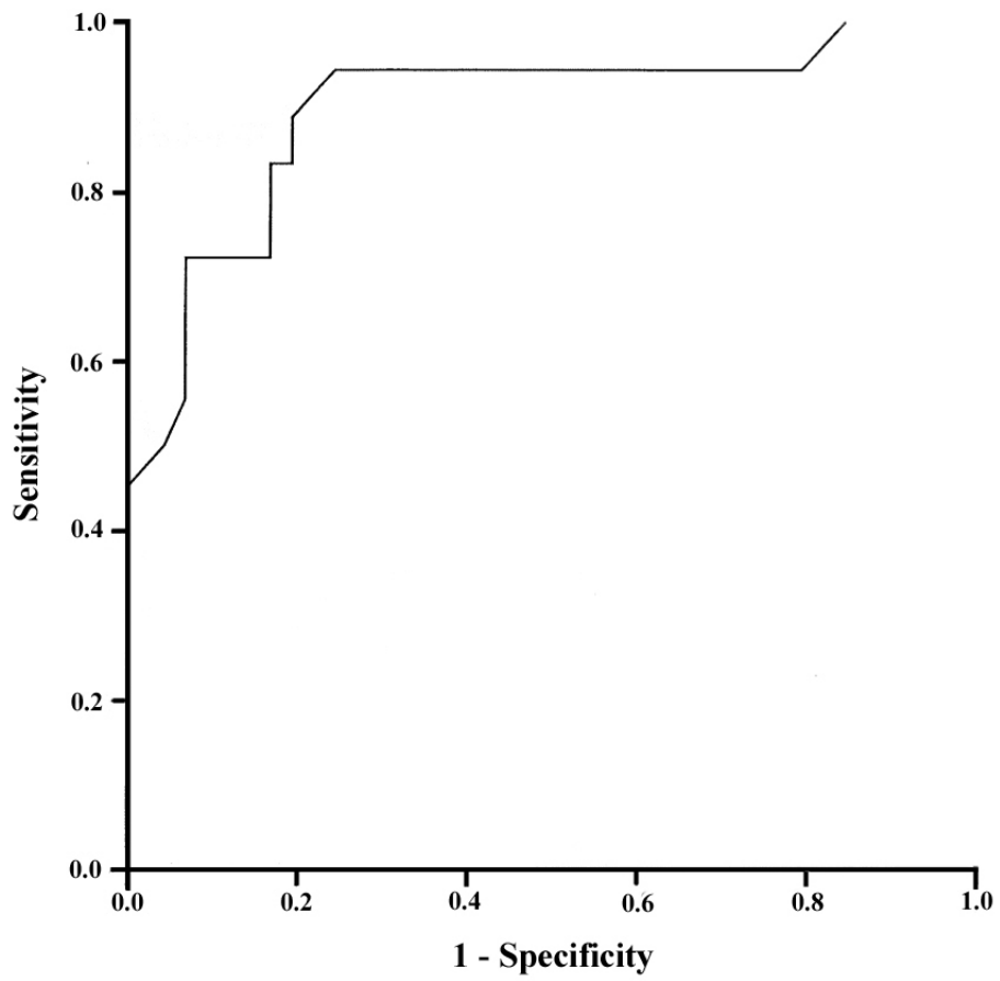
Figure 1b. Receiver operating characteristic curve: processing speed for healthy subjects versus visual neglect (N+) patients in star cancellation task.
