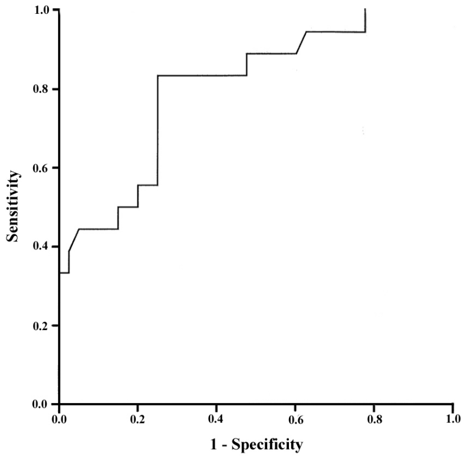
Figure 1a. Receiver operating characteristic curve: processing speed for healthy subjects versus visual neglect (N+) patients in letter cancellation task.
