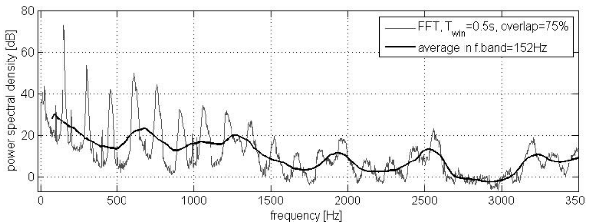
Fig. 6. Spectra of the acoustic signal measured outside the human vocal tract during phonation into the tube. Thick and thin lines respectively denote the “filtered spectrum” and the FFT spectrum.
