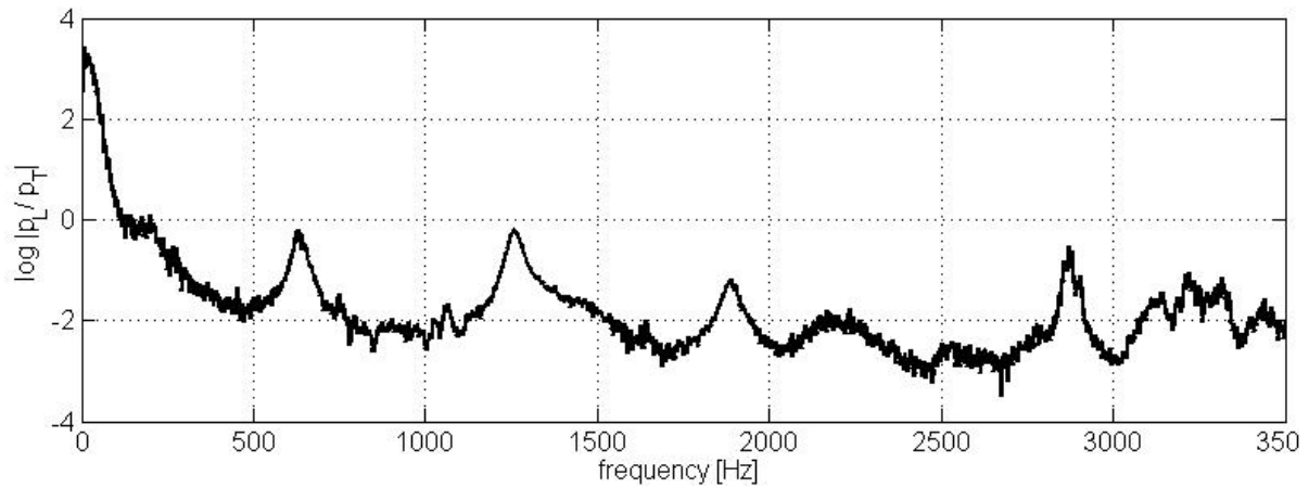
Fig. 9. A measured transfer function between the lips and the open tube end for the human vocal tract prolonged by the tube and excited by random noise from the loudspeaker.
