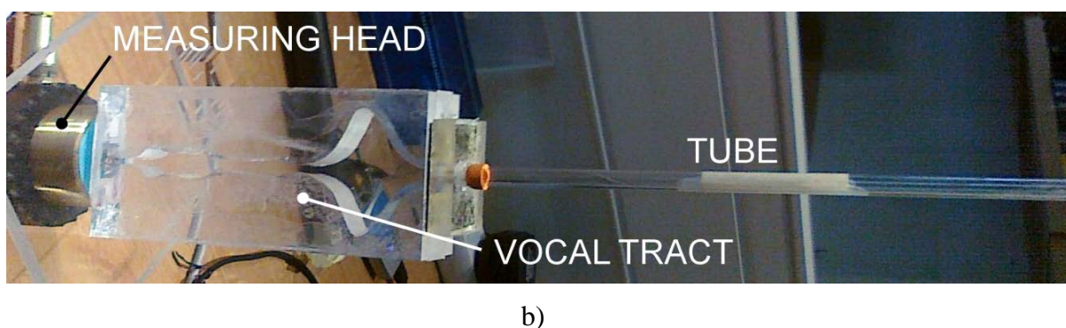
Fig. 4. (a) A layout of the measuring head of the BIAS 6 system [16] (reproduced with permission of Prof. Gregor Widholm) and (b) experimental setup for measuring the acoustic input impedance on a plexiglass model of the vocal tract prolonged by a tube and installed in the measuring head of the system BIAS 6 at the position of the vocal folds.
