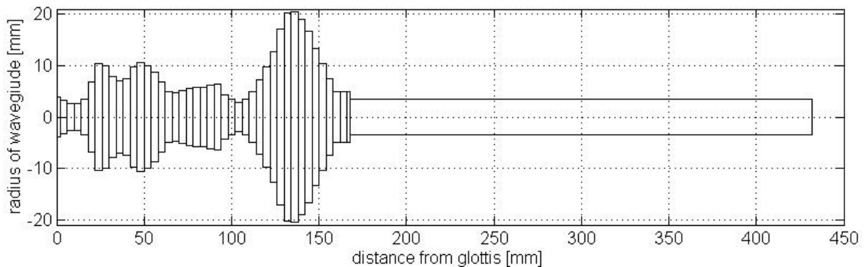
Fig. 5. Geometry of the VT model prolonged by the tube.
