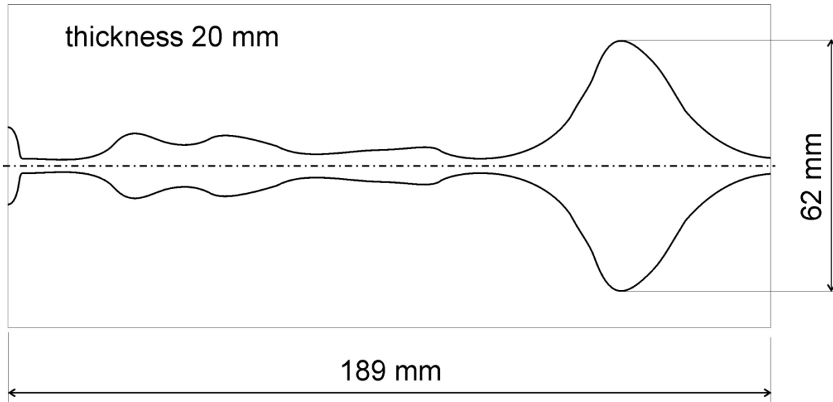
Fig. 3. Geometry of the plexiglass VT model.
