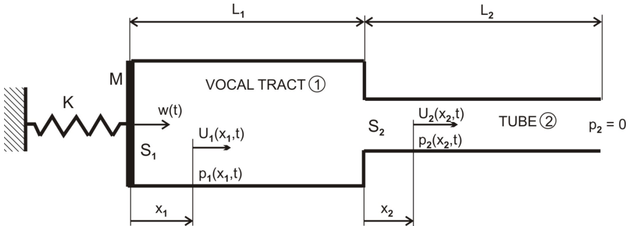
Fig. 13. Simplified model of the vocal tract prolonged by a tube and closed with a yielding wall.
