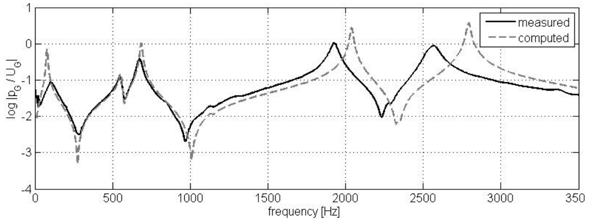
Fig. 11. A comparison of measured (solid line) and computed (dashed line) magnitudes of the input impedance p_G/U_G for the artificial plexiglass vocal tract model prolonged by the tube.
