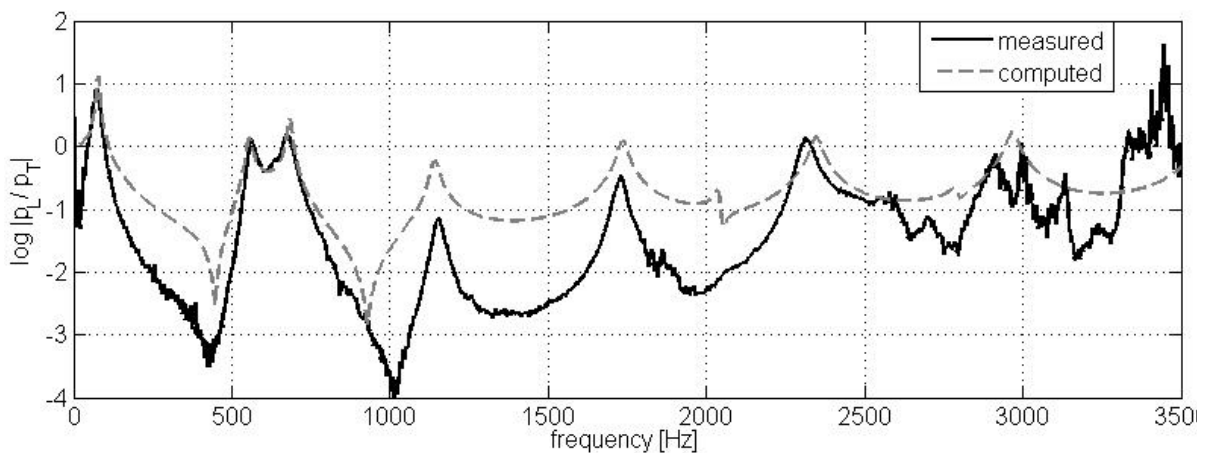
Fig. 10. A comparison of measured (solid line) and computed (dashed line) transfer functions p_L/p_T between the lips and the open tube end for the plexiglass vocal tract
