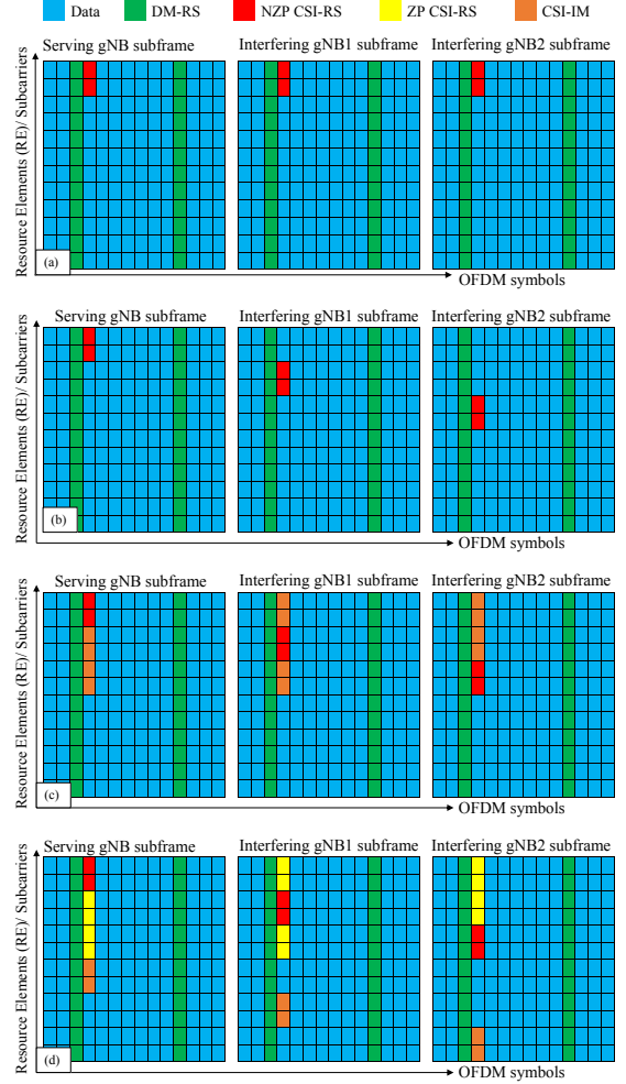
Fig. 2: Illustration of different CSI-RS configurations enabling non-precoded (a and c), or precoded (b and d) interference measurement through using either NZZ CSI-RS method (a and b) or CSI-IM method (c and d).
