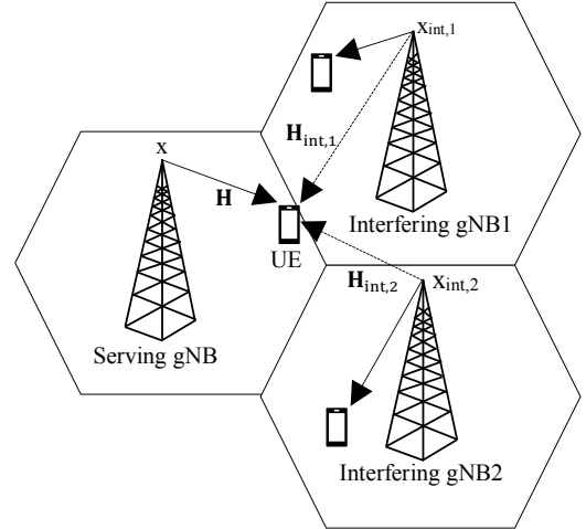
Fig. 1: Interference model consists of one serving cell and two interfering cells. Here x , x_{int,1} and x_{int,2} correspond to the transmitted symbols from serving and interfering gNBs respectively, and H , H_{int,1} and H_{int,2} correspond to the channel responses of the received signals for each relevant subcarrier index.
