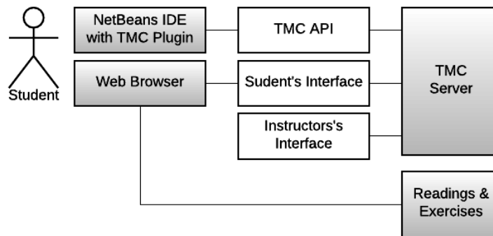
Figure 1. Architecture of MOOC.
