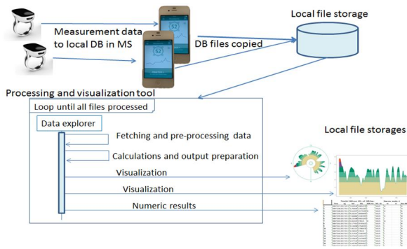
Fig. 1 Process of EDA data processing and visualization.
